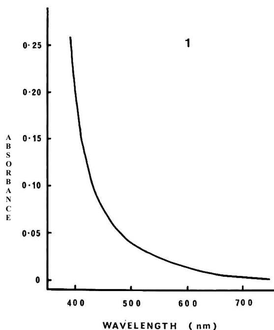
FIGURE 1 Spectrum of a wine showing no pinking (from Simpson, 1977).
