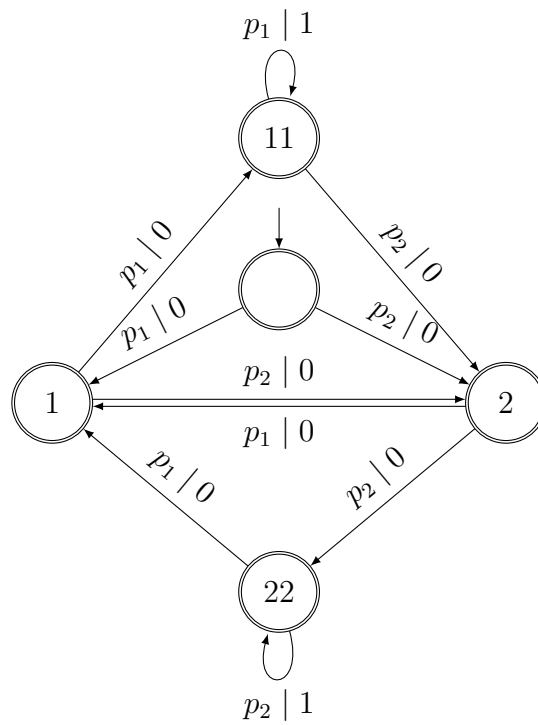
Figure 2: Transducer detecting 3-runs of any letter.
