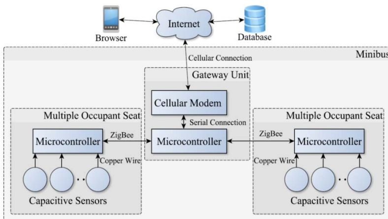
Figure 1 Occupancy detection system with online reporting in real time
