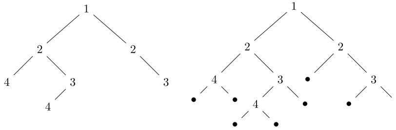
Fig. 1. Left: a weakly increasing tree with 7 nodes and 4 distinct labels; Right: its associated completed tree.
