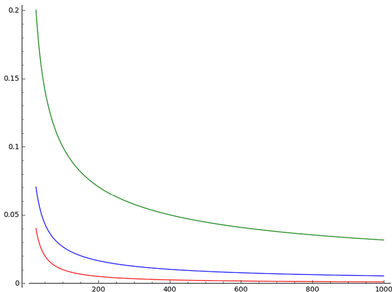
Fig. 2. The blue curve corresponds to the function n \mapsto B_n/((\ln 2)^{-n}(n-1)!) . (For interpretation of the references to color in this figure legend, the reader is referred to the web version of this article.)
