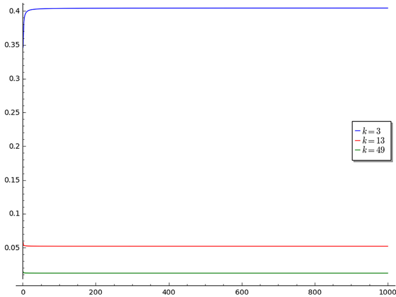
Fig. 3. The normalization of B_n and their asymptotic behaviors for k = 3, 13, 49 .
