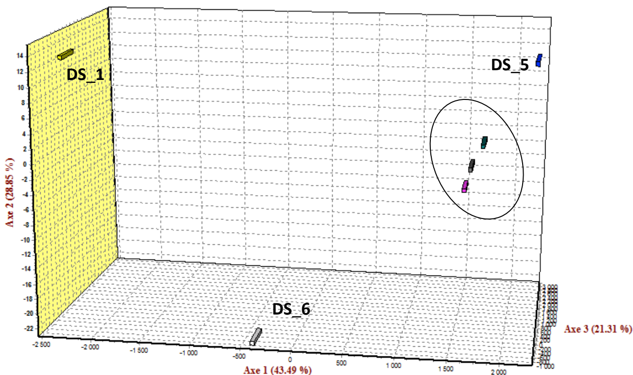
Figure 2. Factorial component analysis (FCA) based on 31 SNP loci in six H. midae populations. The respective populations are indicated by color: Family DS_1 (Yellow), Family DS_5 (Blue), Family DS_6 (White), Riet Point (Grey), Saldanha Bay (Pink) and Witsand (Green). The wild populations are encircled.
