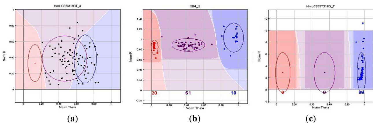
Figure 1. Genoplots obtained with the GenomeStudio™ Genotyping Module representative of (a) a failed SNP; (b) a successfully genotyped (polymorphic) SNP; and (c) a monomorphic SNP analyzed in this study.
