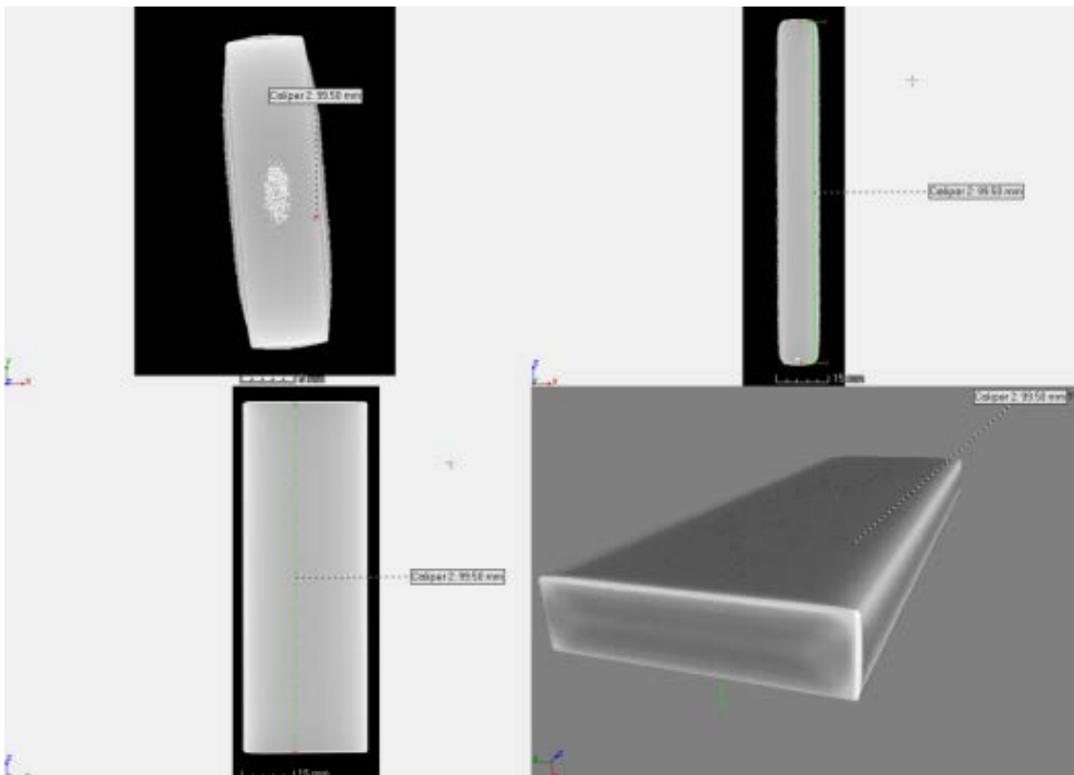
Figure 5: Dimensional measurement using the VG Studio Max calipers function
