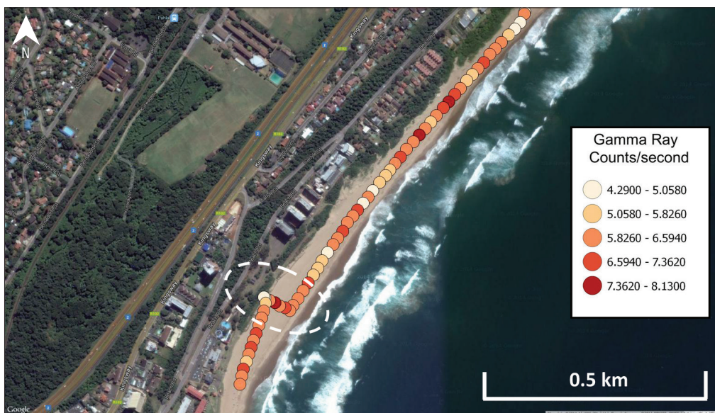
Figure 6: A Google Earth image indicating the relative potassium concentrations on the north beach of Amanzimtoti, South Africa. The colour graded overlay displays the gamma ray counts in the region of interest around the 1460.8 keV gamma ray emission.
