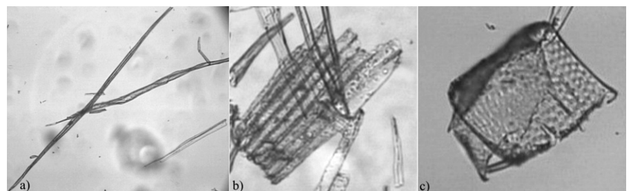
Fig. 2. Different cell types of A. mearnsii as seen through a transmission microscope: a, fibres; b, parenchyma cells; c, vessel element; x50 magnification. AFM analysis was subsequently performed on surfaces of each cell type.
