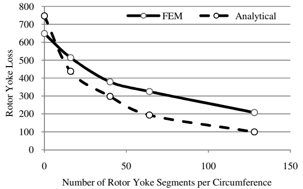
Fig. 12: Analytical and FE calculated rotor yoke loss versus level of rotor yoke partial segmentation and 17.5% penetration.
