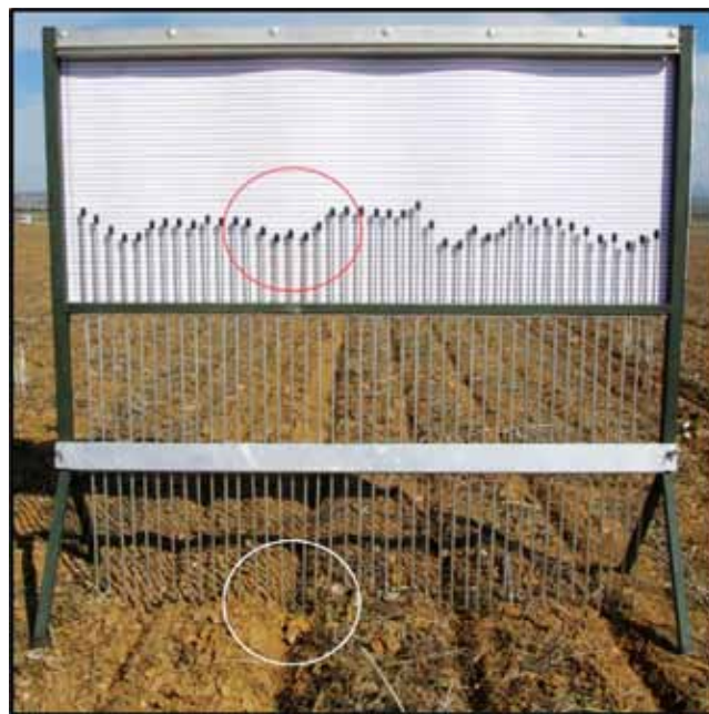
Fig. 2. Pin profiler used to determine the amount of aboveground soil disturbance. The white circle at the bottom indicate the furrow in the soil caused by the opener, while the red circle at the top indicates the roughness profile of the furrow.
