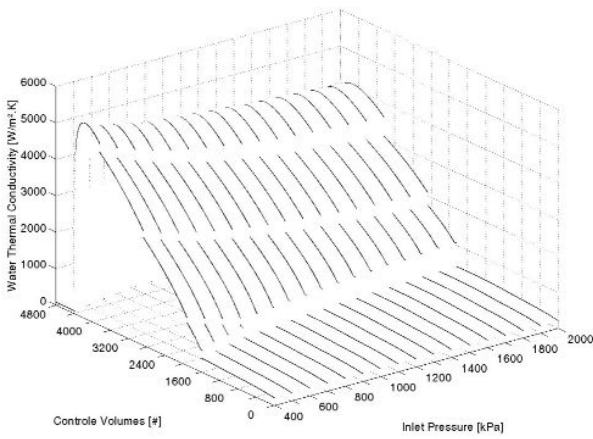
Figure 11: Water thermal heat transfer coefficient
