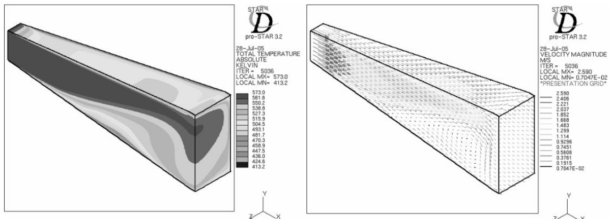
Figure 6: (left) A sectional temperature distribution through a diffuser (right) A sectional velocity field through a diffuser
