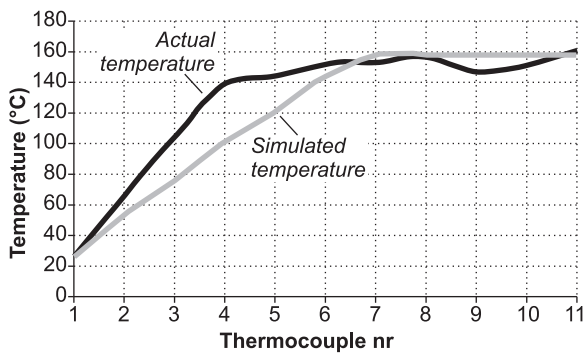
Figure 4: Actual versus simulated temperatures inside the heat exchanger
