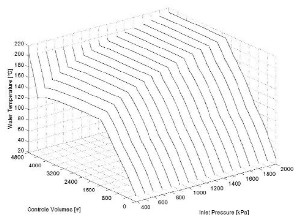
Figure 10: Water temperature distribution
