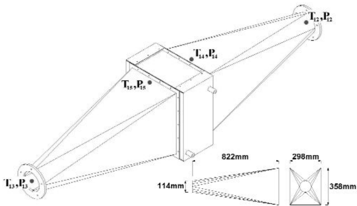
Figure 3: Measurements taken on the exhaust inlet ducting
