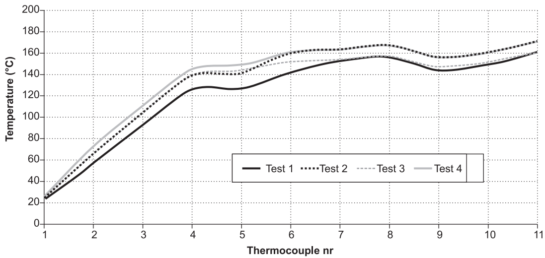
Figure 7: Test point comparisons
