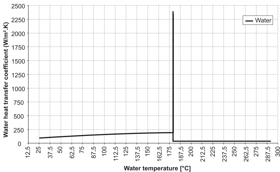
Figure 12: Water heat transfer coefficient vs. temperature
