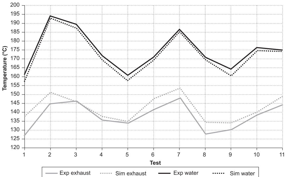
Figure 8: Actual and simulated outlet temperatures
