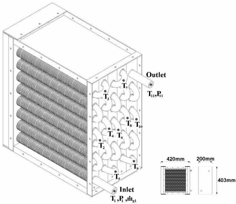
Figure 2: Measurements taken on the heat exchanger
