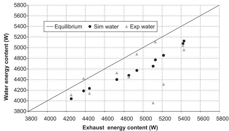
Figure 9: Heat exchanger experimental and simulated energy balance
