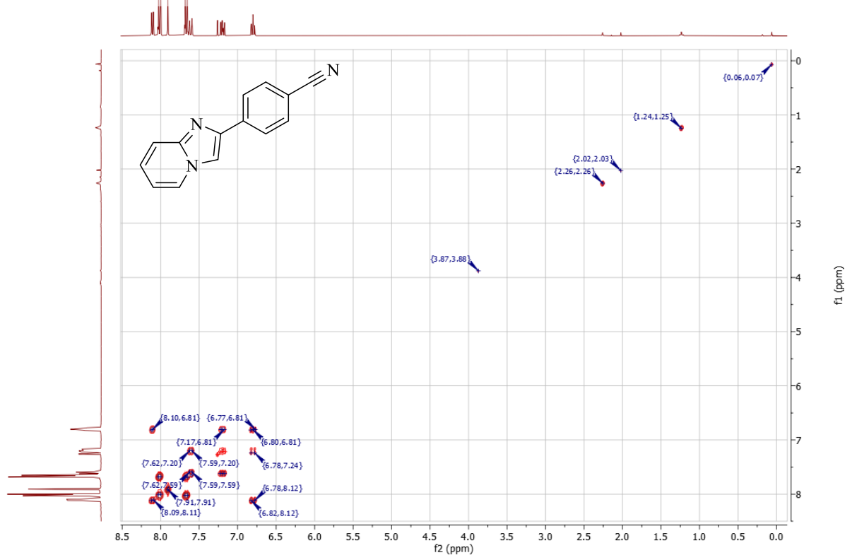
COSY NMR spectrum
