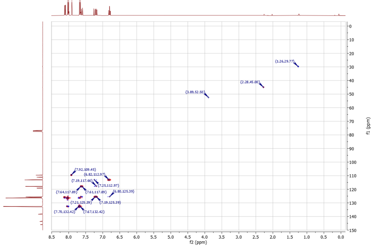
HSQC NMR spectrum
