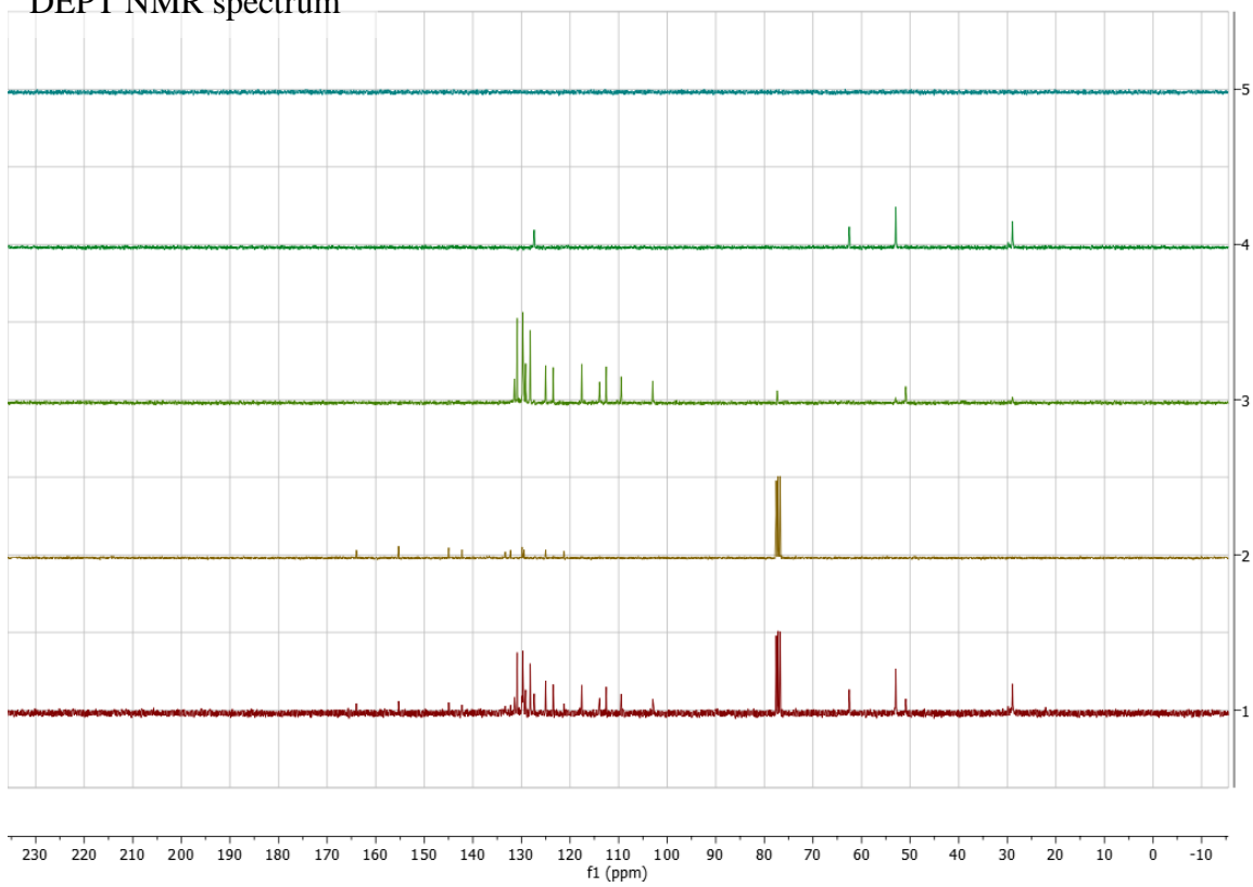
DEPT NMR spectrum
