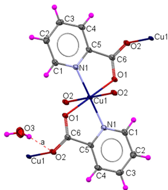
Fig. 1 Thermal ellipsoid plot (ORTEP) view of CP-1 showing all atoms and numbering
