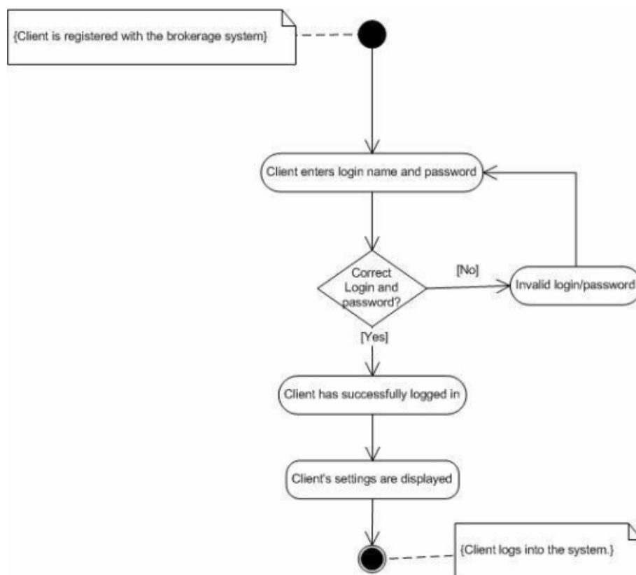
Figure 3.1: An example of an activity diagram showing a high level website login algorithm (Lucidchart - Activity Diagram Introduction Page, 2015).
