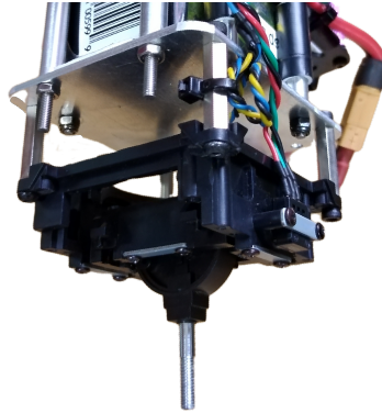
Figure 6.3: Payload angle sensor with linear potentiometers.
