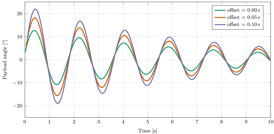
Figure 7.8: White-box predictions from different initial conditions for a dynamic payload ( m_1 = 0.2 kg, l_1 = 0.5 m, m_2 = 0.1 kg, l_2 = 0.6 m).
