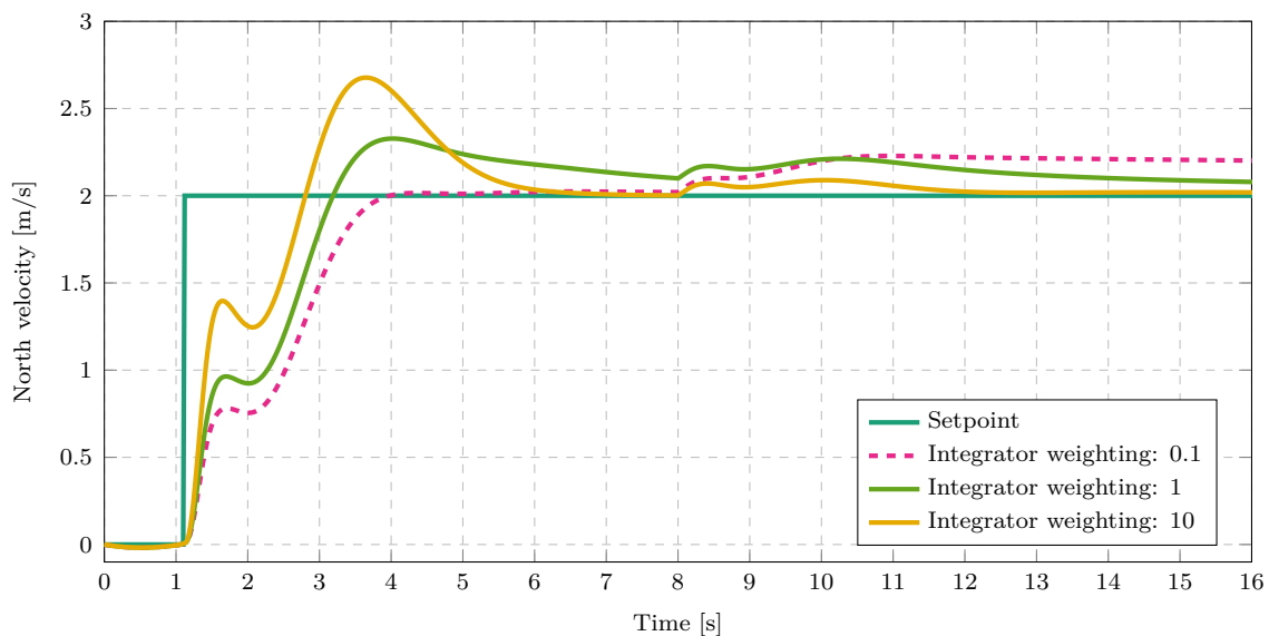
Figure 5.17: Different LQR responses for different integrator gains ( l = 2 m, m_p = 0.3 kg).
