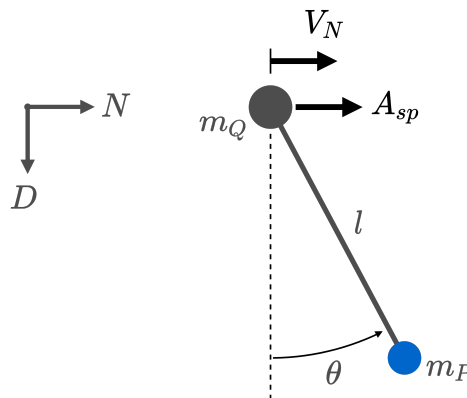
Figure 4.1: Schematic of a floating pendulum model considered for a North velocity controller.
