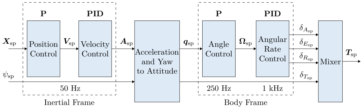
Figure 5.1: Cascaded PID control architecture of PX4 [7].
