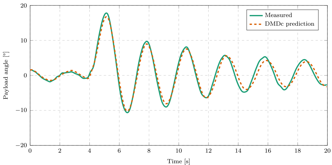
Figure 7.13: Model predictions of practical flight data with a suspended payload for a North velocity step input ( l = 2 m, m_p = 0.3 kg).
