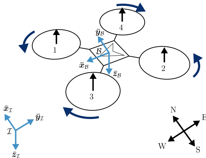
Figure 3.1: Inertial and body coordinate frames of a quadrotor [6].
