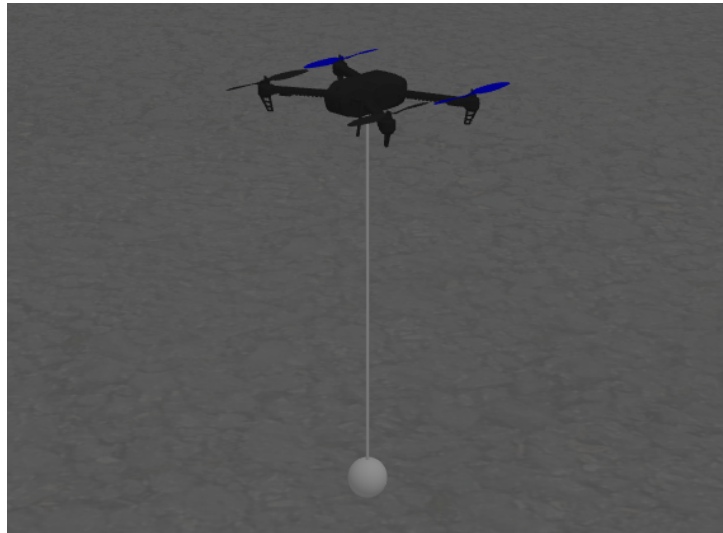
Figure 6.5: Model of Honeybee in the Gazebo simulator.
