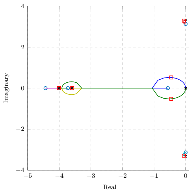
Figure 5.5: Root locus plot of the North velocity dynamics including PID controller.
