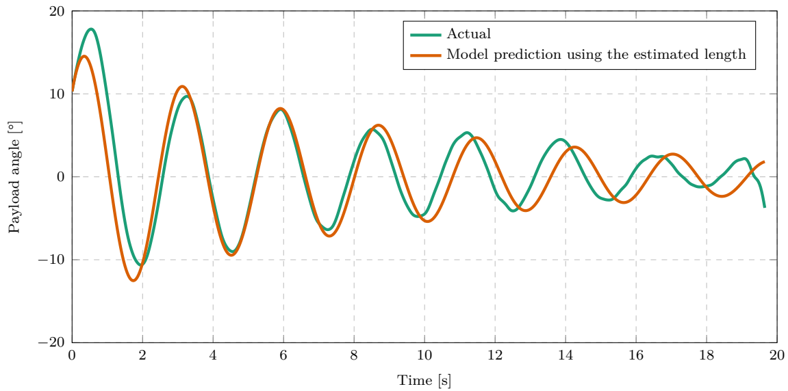
Figure 7.2: White-box model prediction for a North velocity step input ( l = 2 m, m_p = 0.3 kg.).
