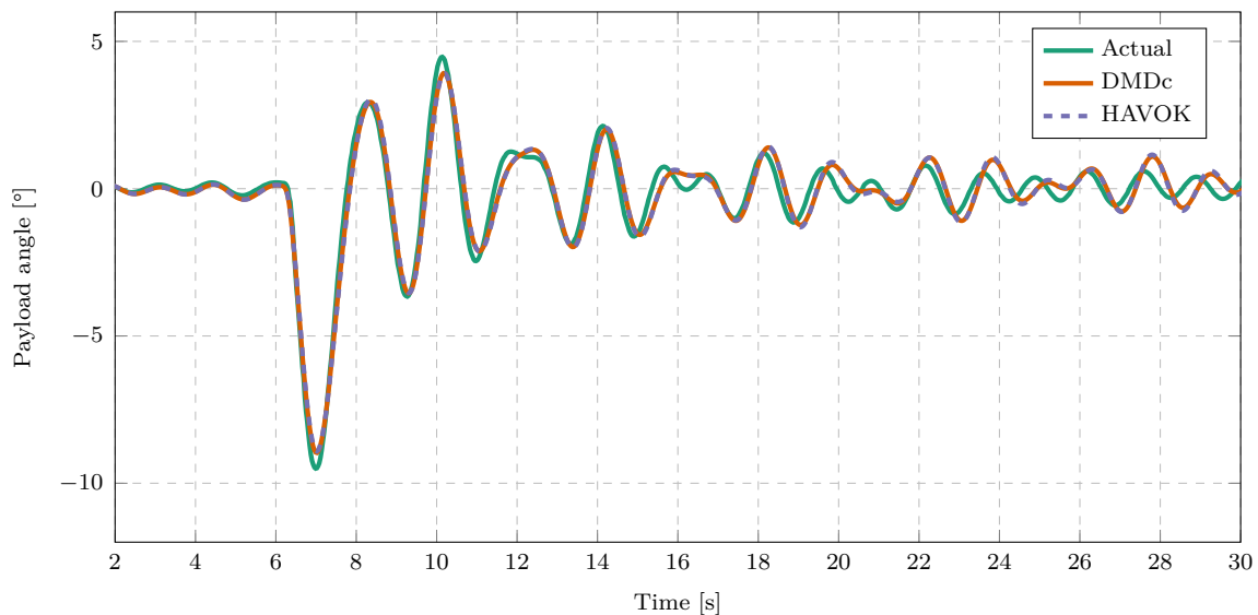
Figure 4.19: Data-driven model predictions of a double pendulum for a North velocity step input ( m_1 = 0.2 kg, l_1 = 1 m, m_2 = 0.1 kg, l_2 = 0.3 m).
