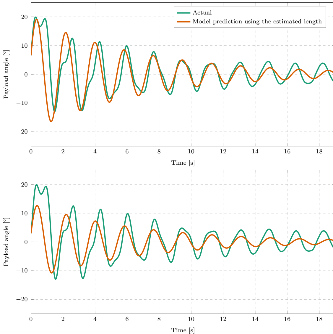
Figure 7.7: Data predictions using slightly different initial conditions for a velocity step response with a dynamic payload ( m_1 = 0.2 kg, l_1 = 0.5 m, m_2 = 0.1 kg, l_2 = 0.6 m).
