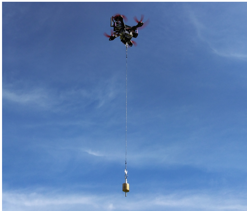
Figure 6.8: Practical flight with Honeybee and a suspended payload.
