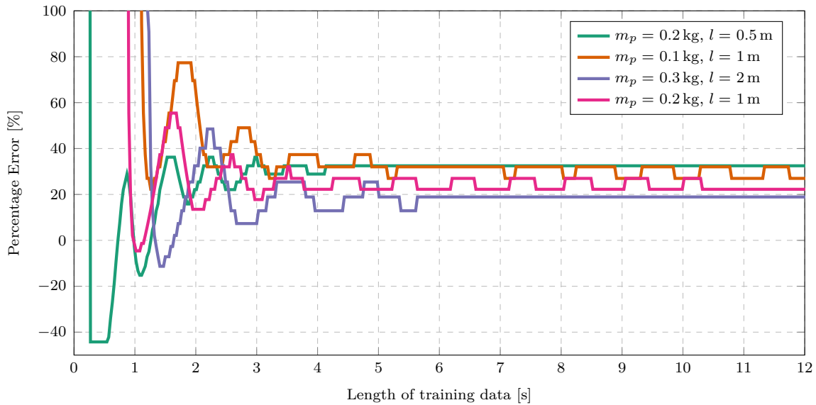
Figure 7.1: Plot of the error in cable length estimation as a function of length of training data (wind speed \approx 0.5 m/s).
