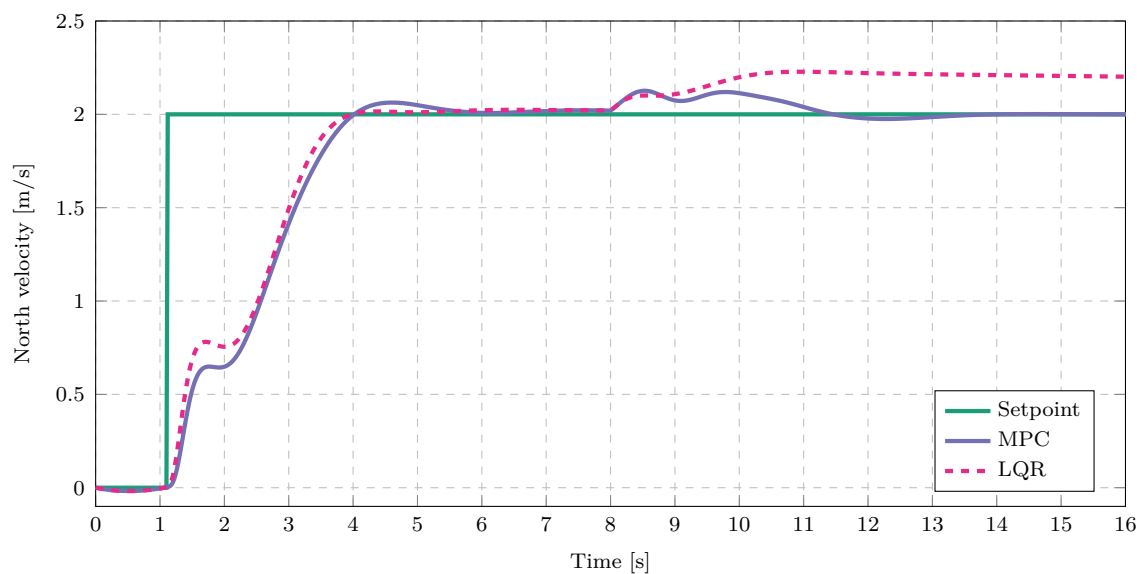
Figure 5.16: Effect of an unmeasured step input disturbance. ( l = 2 m, m_p = 0.3 kg).
