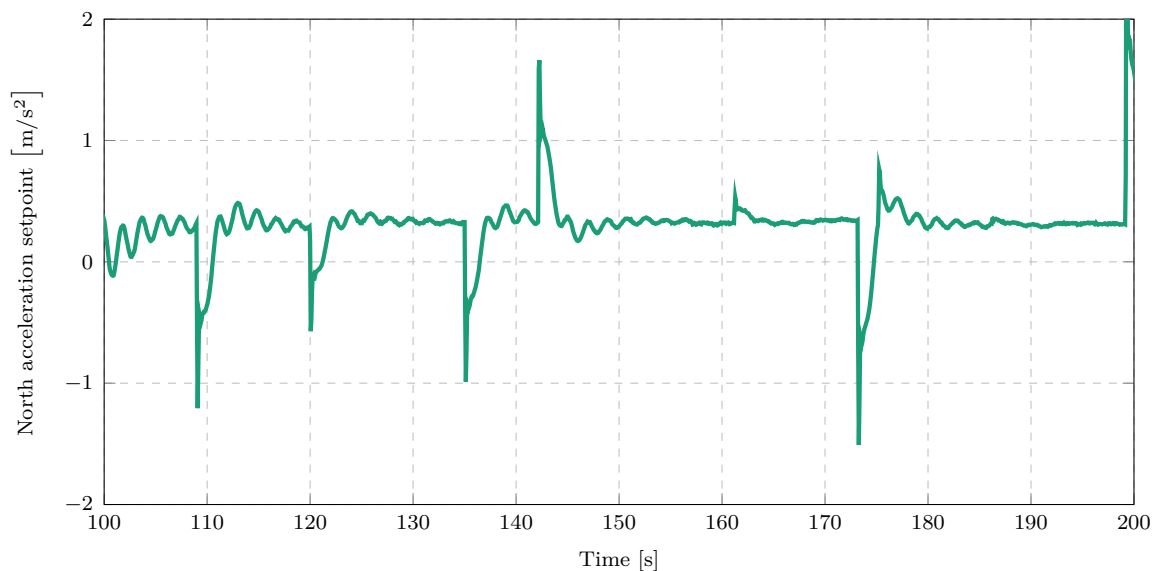
Figure 4.10: Acceleration setpoint training data from random velocity step inputs ( m_p = 0.2 kg, l = 1 m).
