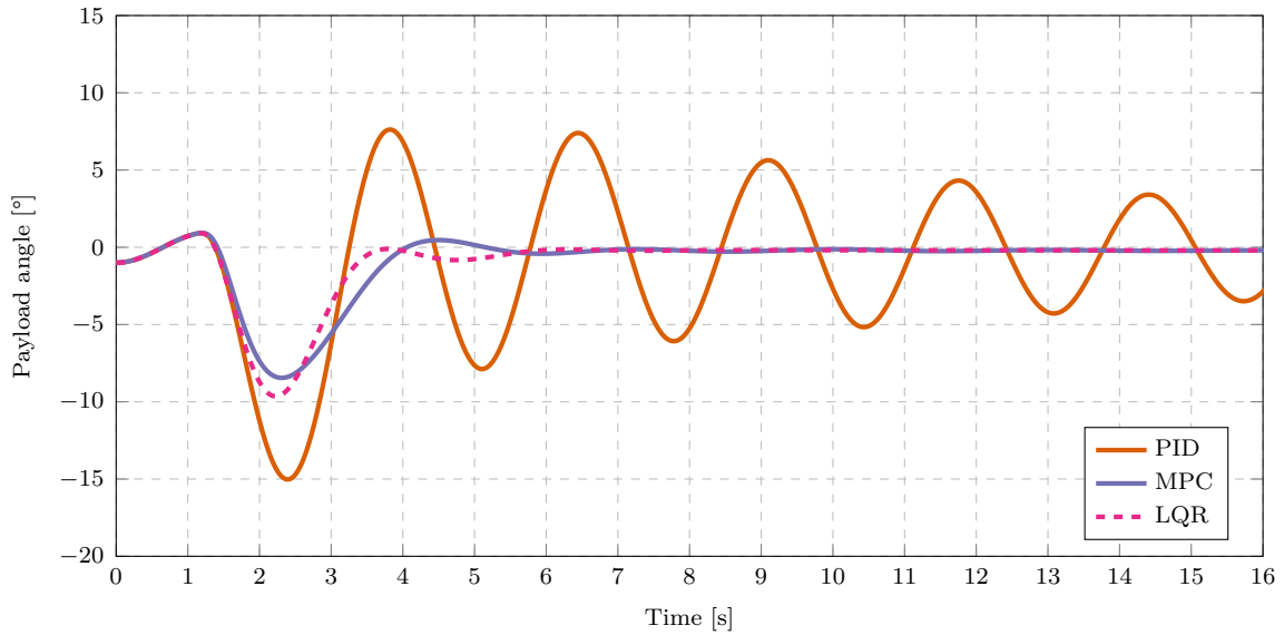
Figure 5.12: Payload angle comparison of different controllers ( l = 2 m, m_p = 0.3 kg).
