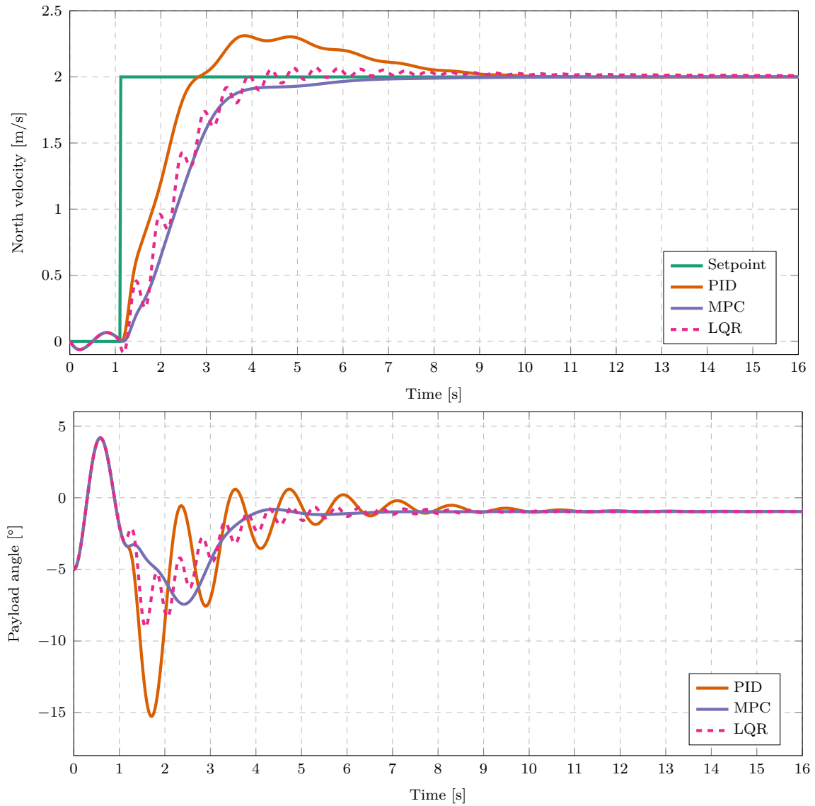
Figure 5.22: Velocity step responses with the multirotor mass decreased by 0.25 kg ( l = 0.5 m, m_p = 0.3 kg).
