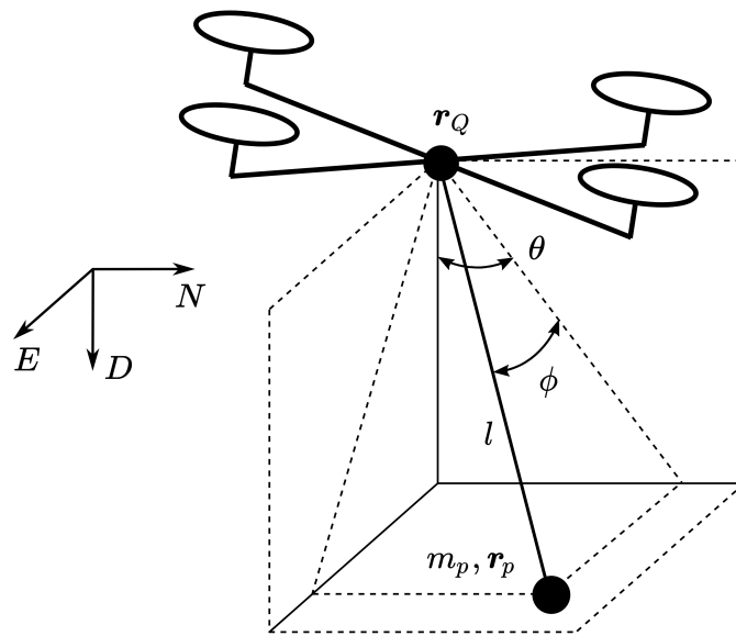
Figure 3.3: Schematic of a multirotor with suspended payload [2].
