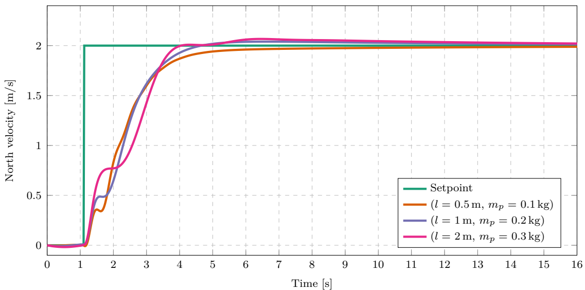
Figure 5.7: LQR velocity step responses with different payloads.
