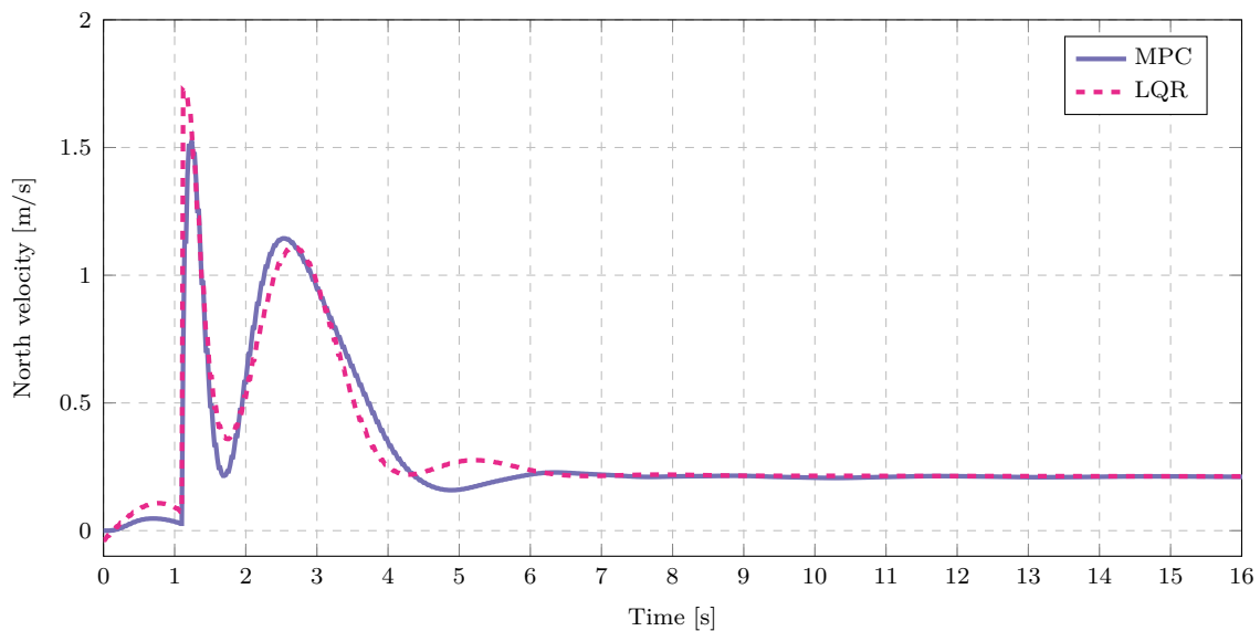
Figure 5.13: Acceleration setpoint commanded by different controllers for a velocity step input ( l = 2 m, m_p = 0.3 kg).
