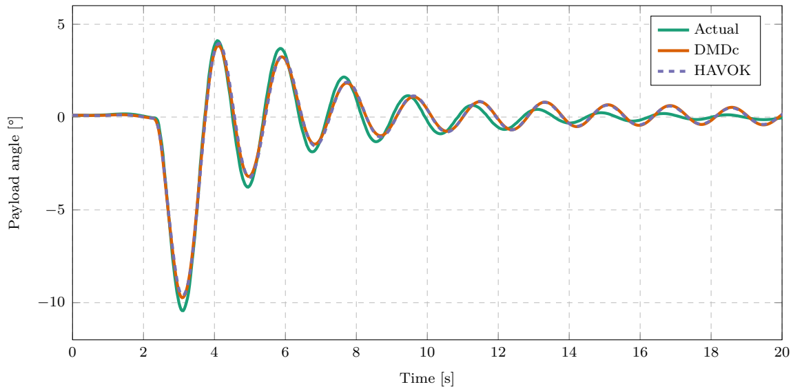
Figure 4.18: Data-driven model predictions of a single pendulum for a North velocity step input ( m_p = 0.3 kg, l = 1 m).
