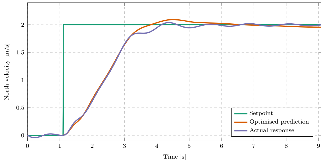
Figure 5.20: Optimised prediction and actual velocity response of the MCP with a dynamic payload.
