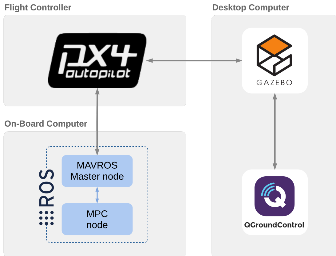
Figure 6.7: Different software and hardware components of a HITL simulation.
