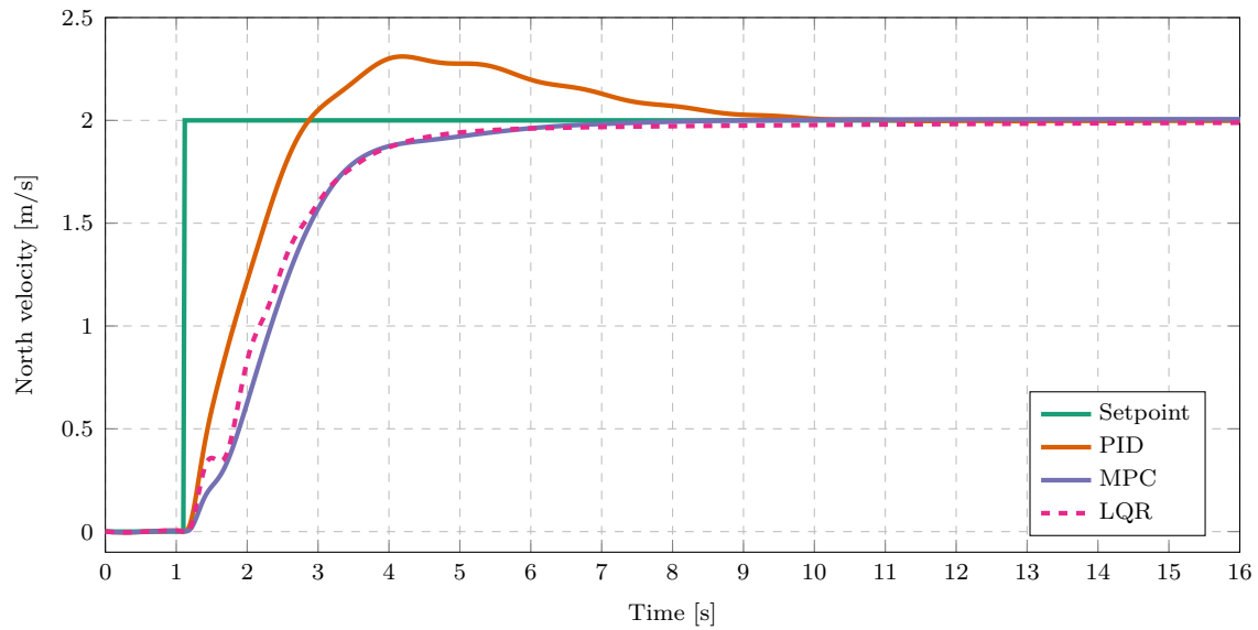
Figure 5.15: Velocity step response comparison of different controllers ( l = 0.5 m, m_p = 0.1 kg).
