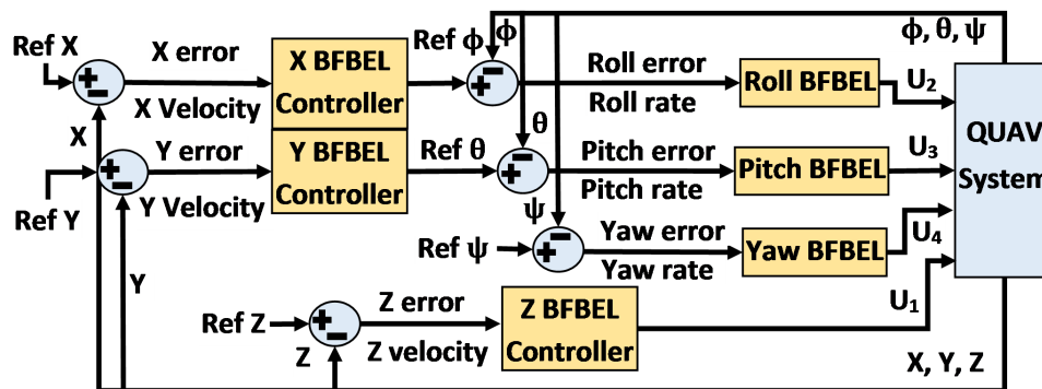
Figure 2.6: Controller structure proposed by Muthusamy et al. [5].
