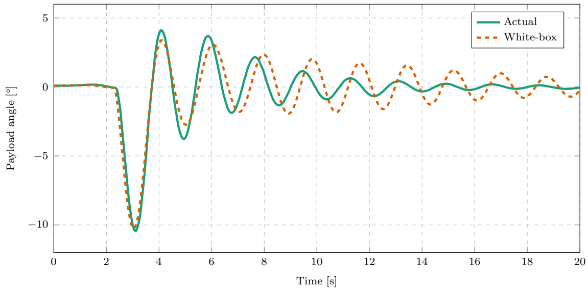
Figure 4.15: White-box model predictions of a single pendulum for a North velocity step input ( l = 1 m, m_p = 0.3 kg).
