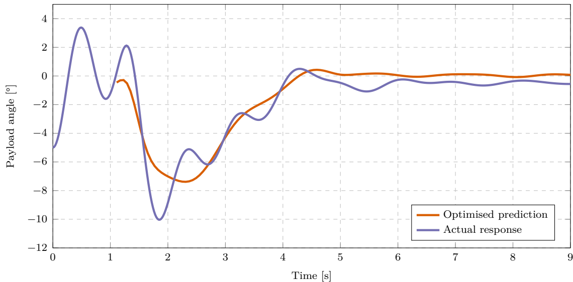
Figure 5.21: Optimised prediction and actual payload angle response of the MPC with a dynamic payload.
