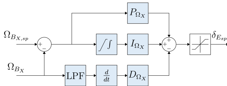
Figure 5.2: Angular rate controller diagram [7].
