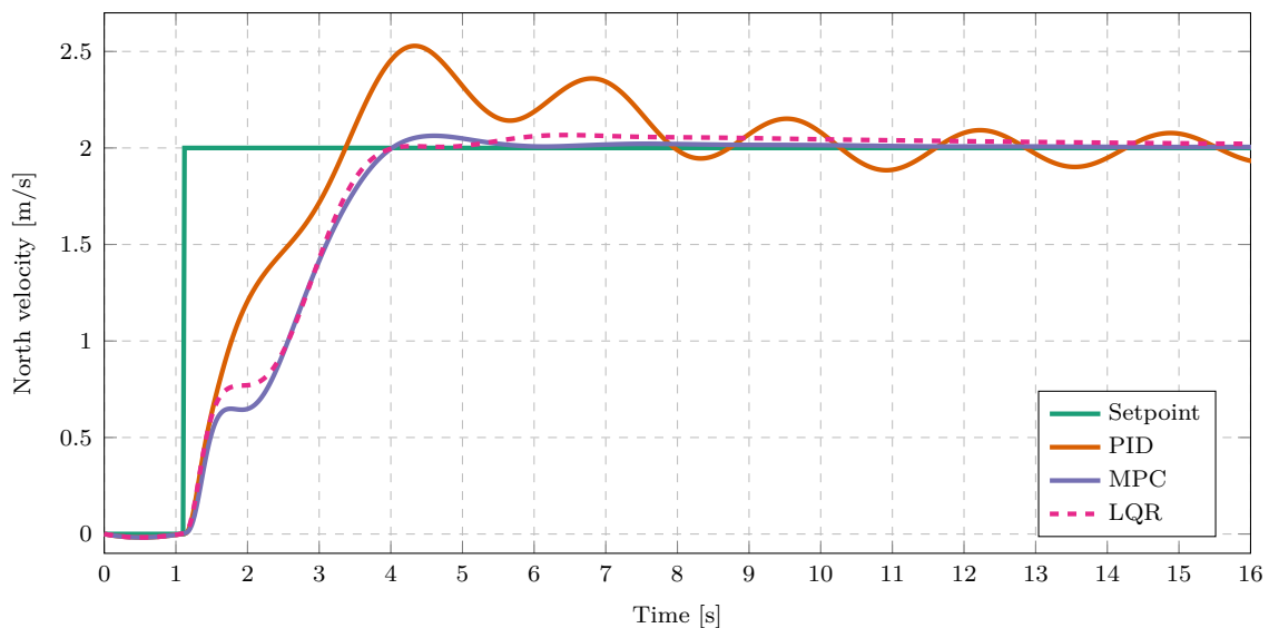
Figure 5.11: Velocity step response comparison of different controllers ( l = 2 m, m_p = 0.3 kg).
