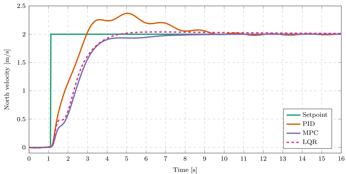
Figure 5.14: Velocity step response comparison of different controllers ( l = 1 m, m_p = 0.2 kg).
