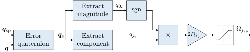
Figure 5.3: Quaternion based angle controller diagram [7].
