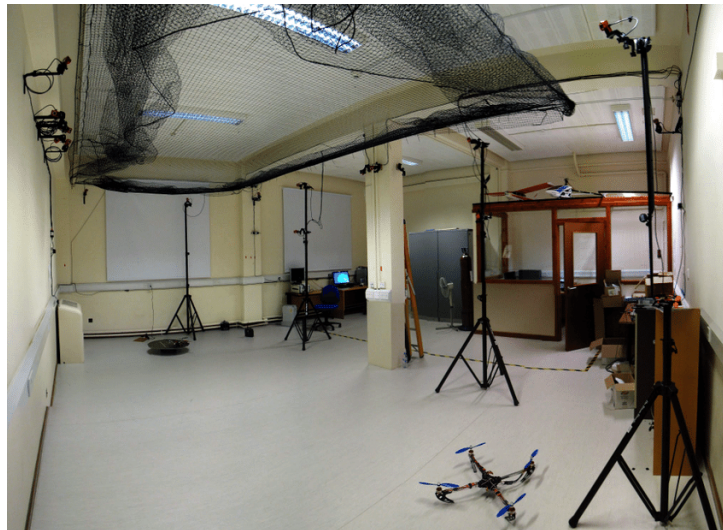
Figure 2.4: Optitrack motion capture system for multirotor experiments [3].
