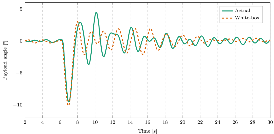
Figure 4.16: White-box model predictions of a double pendulum for a North velocity step input ( m_1 = 0.2 kg, l_1 = 1 m, m_2 = 0.1 kg, l_2 = 0.3 m).
