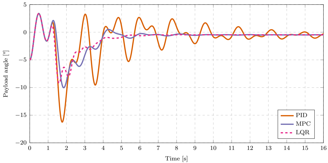
Figure 5.19: Payload angle comparison of different controllers ( l = 2 m, m_p = 0.3 kg).
