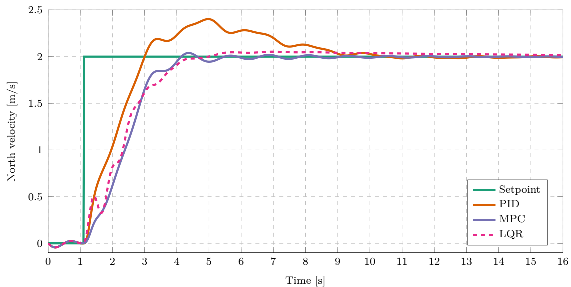
Figure 5.18: Velocity step response comparison of different controllers ( l = 2 m, m_p = 0.3 kg).
