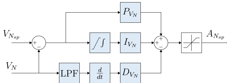
Figure 5.4: Velocity controller diagram [7].
