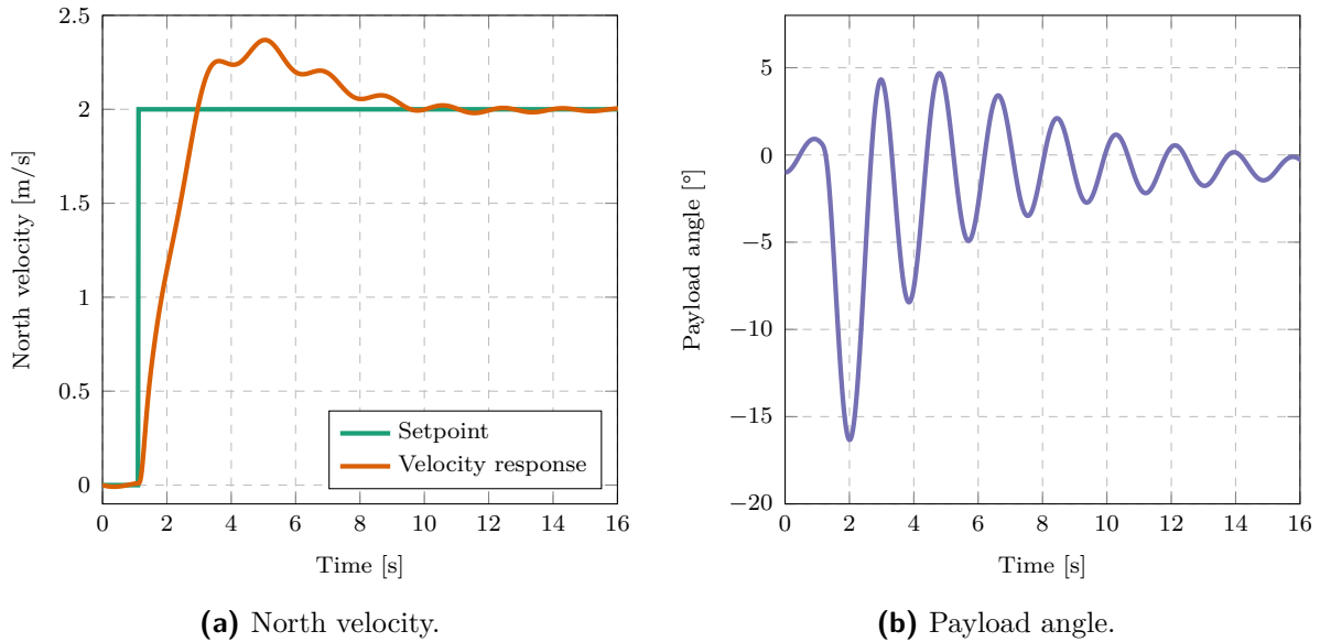
Figure 5.6: PID velocity step response ( l = 1 m, m_p = 0.2 kg).
