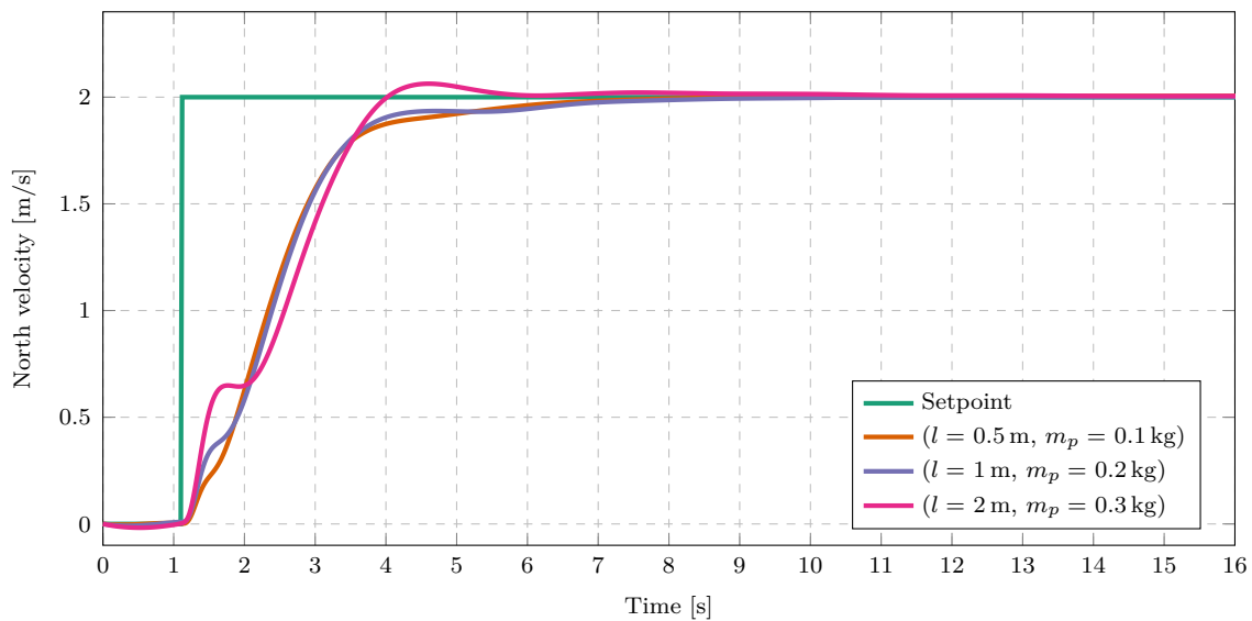
Figure 5.10: MPC velocity step responses with different payloads.
