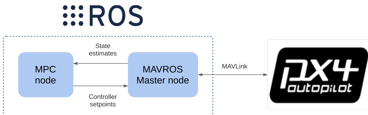
Figure 6.6: Communication between ROS, flight-stack, simulator, and ground station [10].
