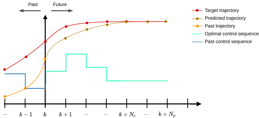
Figure 5.9: Illustration of the receding horizon of an MPC [8].
