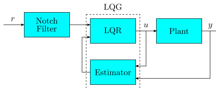
Figure 2.3: Notch filter and LQR control architecture [2].
