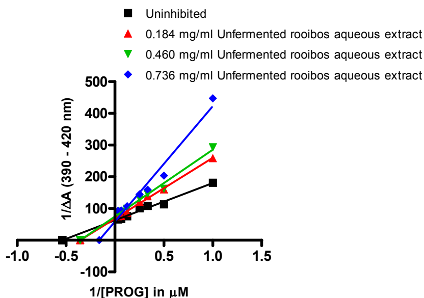
Figure 5.6. Double reciprocal plot of the inhibitory effect of unfermented rooibos aqueous extract on PROG binding. [P450] = 0.8 \mu\text{M} ; [PROG] = 2 - 32 \mu\text{M} ; unfermented rooibos aqueous extract = [0.184 - 0.736 \text{ mg/ml}] . Results are presented as the mean of 3 independent experiments.
