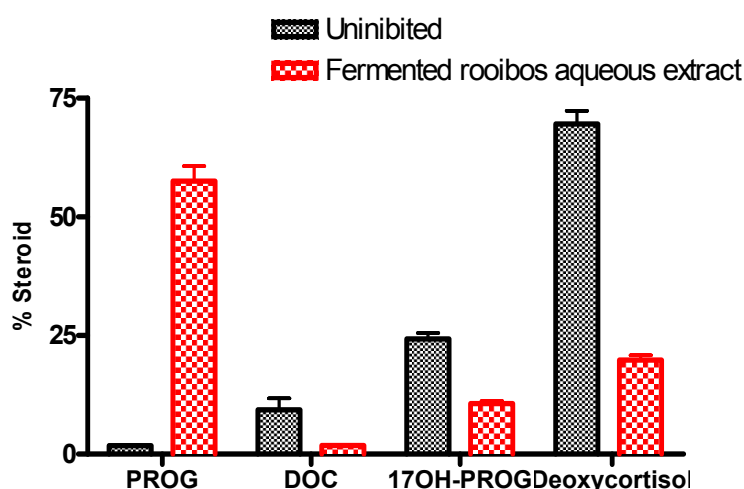
Figure 5.14. Conversion of PROG (10 \mu M) to steroid metabolites DOC, 17OH-PROG and deoxycortisol in the absence and presence of fermented rooibos aqueous extract in ovine adrenal microsomes [ P450 ] = 0.35 \mu M) after initiation with NADPH (1 mM); [Fermented rooibos aqueous extract] = 2.3 mg/ml. Results are presented as the mean, error bars represent SEM and n=3 .
