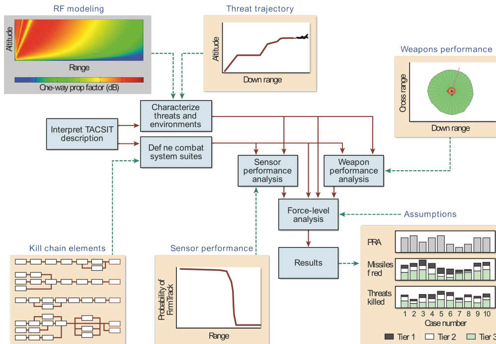
FIGURE 8.2: The “way-ahead” M&S process for the Aegis BMD system [186].
