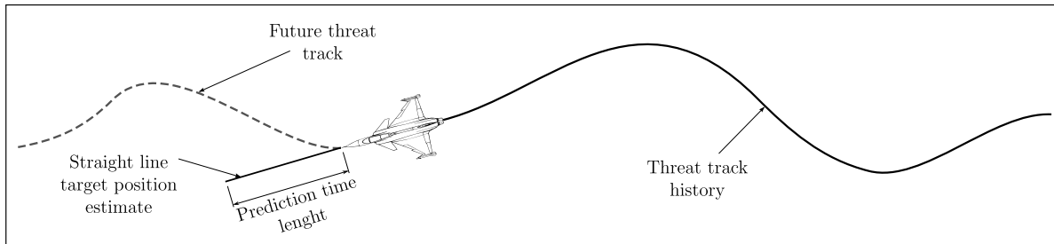
FIGURE 4.6: Flight path prediction method employed.
