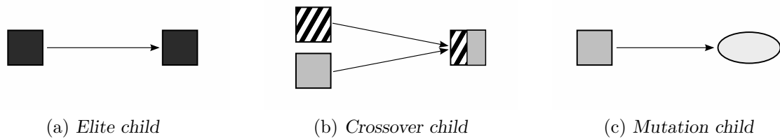
FIGURE 6.1: Three types of children used to populate the next generation in the generic algorithm.
