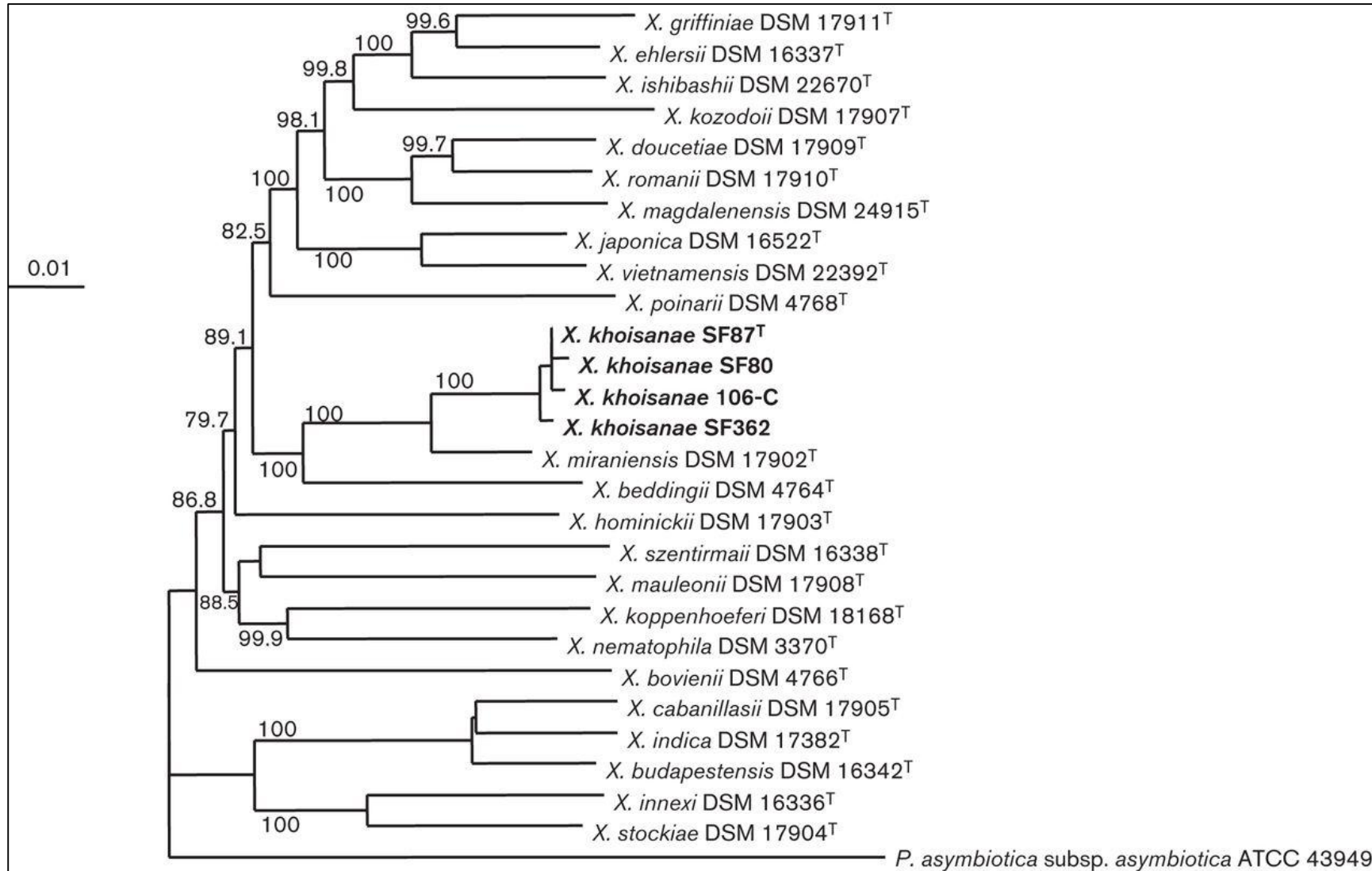
Fig. 1. Phylogenetic relationship of X. khoisanae strains SF87 T , SF80, 106-C and SF362 to known Xenorhabdus species based on concatenated (16S rRNA, recA, dnaN, gltX, gyrB and infB) gene sequences.
