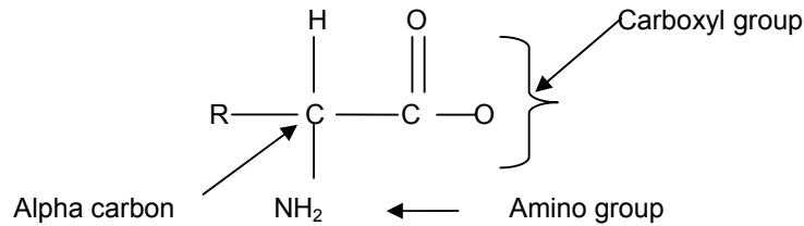
Figure 2 General structure of amino acids.
