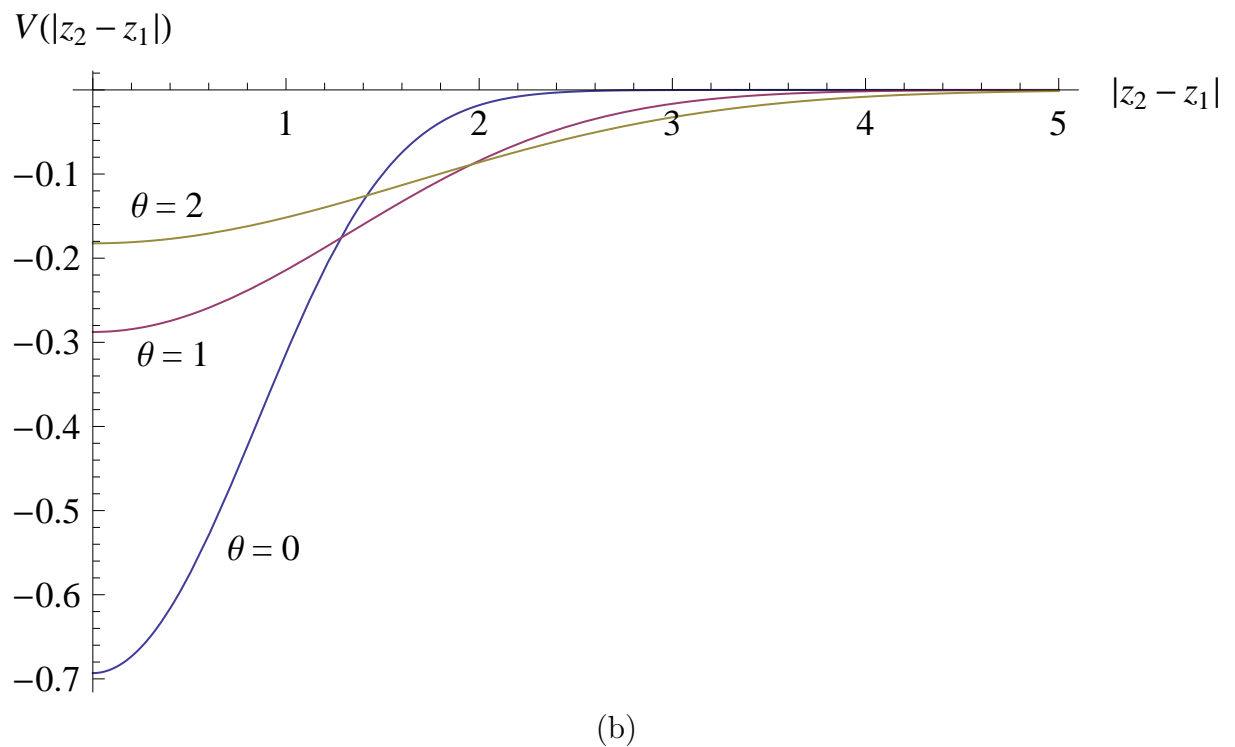
Figure 4.1: The exchange potential for two fermions (a) and two bosons (b) plotted for different values of \theta for fixed \beta ( \beta = \hbar = m = 1 ).
