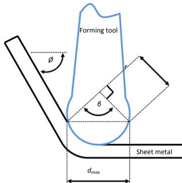
Figure 4: Spindle speed ( \omega ) in terms of feed rate ( v ), tool radius ( r ) and wall angle ( \phi )
