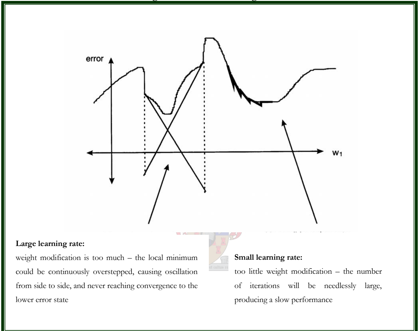
Fig. 4.2 Choice of learning rate
