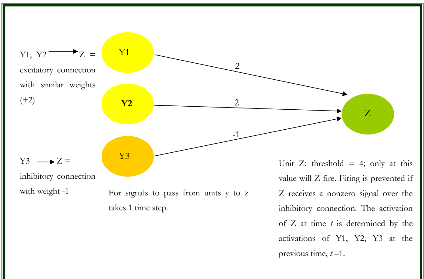
Fig. 2.3 McCulloch-Pitts Neuron
