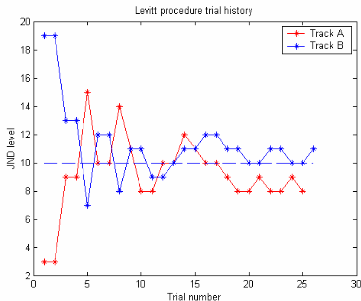
Figure 4.3 A 2-up-1-down, interleaved Levitt procedure
