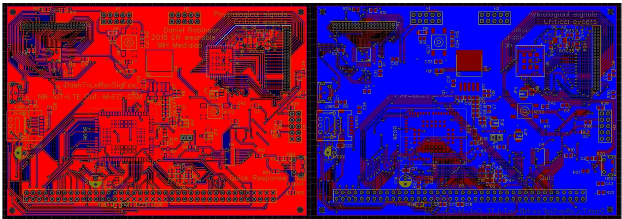
Figure D.6: Top and bottom layout of example PCB
