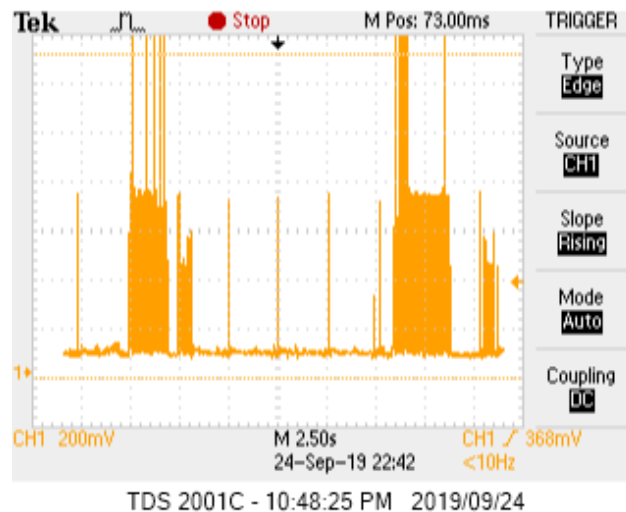
Figure 3.23: An oscilloscope measurement of the Echo test in progress. Notice the four DRX cycles before the second Echo response. Echoes worked successfully every time, and did not take another 2.56 seconds DRX cycle longer than the 10 second delay that the echo server induced.
