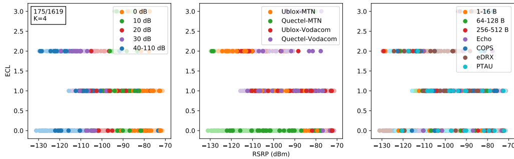
Figure 3.1: ECL levels shown against RSRP for Ublox and Quectel on ZTE-MTN and Nokia-Vodacom networks.
