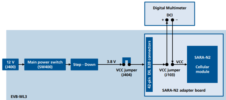
Figure 3.18: Block diagram of current consumption setup for SARA-N2
