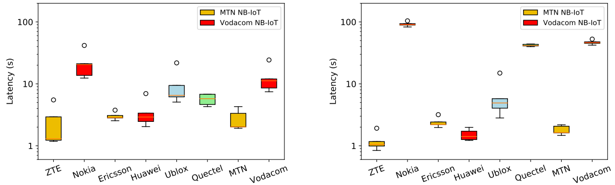
(a) The figure shows measured latency distribution with mean dataset as shown in Appendix A.1.
