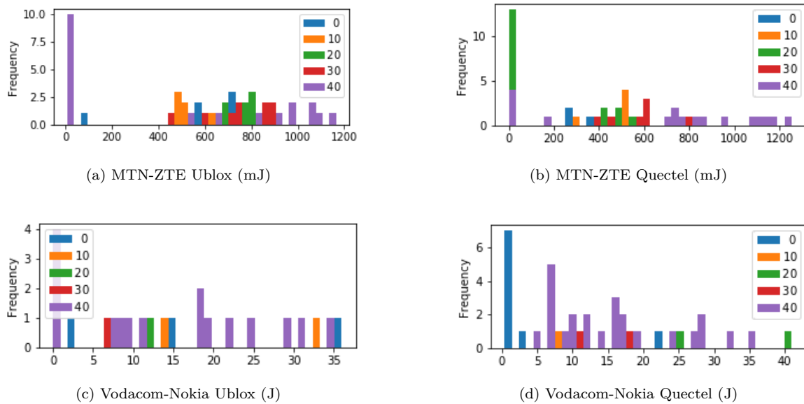
Figure 3.29: PTAU histograms of the energy produced when periodically updating UE devices and networks with tracking area IDs as mentioned in §2.5.5.1. PTAU uses about 20-100 times more power than eDRX for MTE-ZTE and up to 4000 times more energy on Vodacom-Nokia. Frequent PTAU updates should definitely be taken into consideration.
