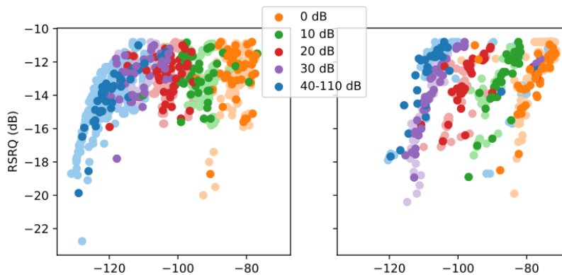
Figure 3.36: RSRQ against RSRP for Ublox and Quectel devices (similar, thus combined) on MTN-ZTE (left) and Vodacom-Nokia (right).
