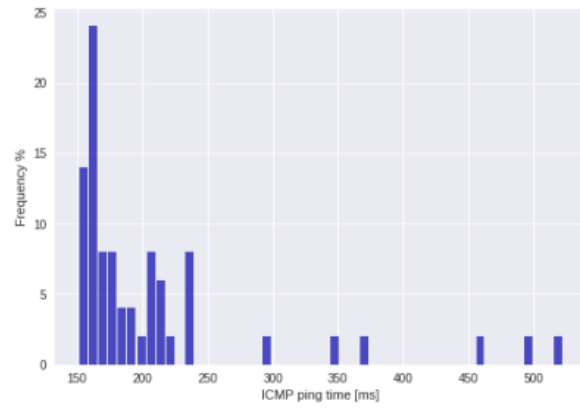
(b) 0 dB attenuation test at Stellenbosch Square R44 intersection at -89 dBm in ECL 0. At the furthest point in Fig. 3.6b, the signal strength increased to -89dBm and resumed a mean of around 209.6ms with a tail around 500ms.
