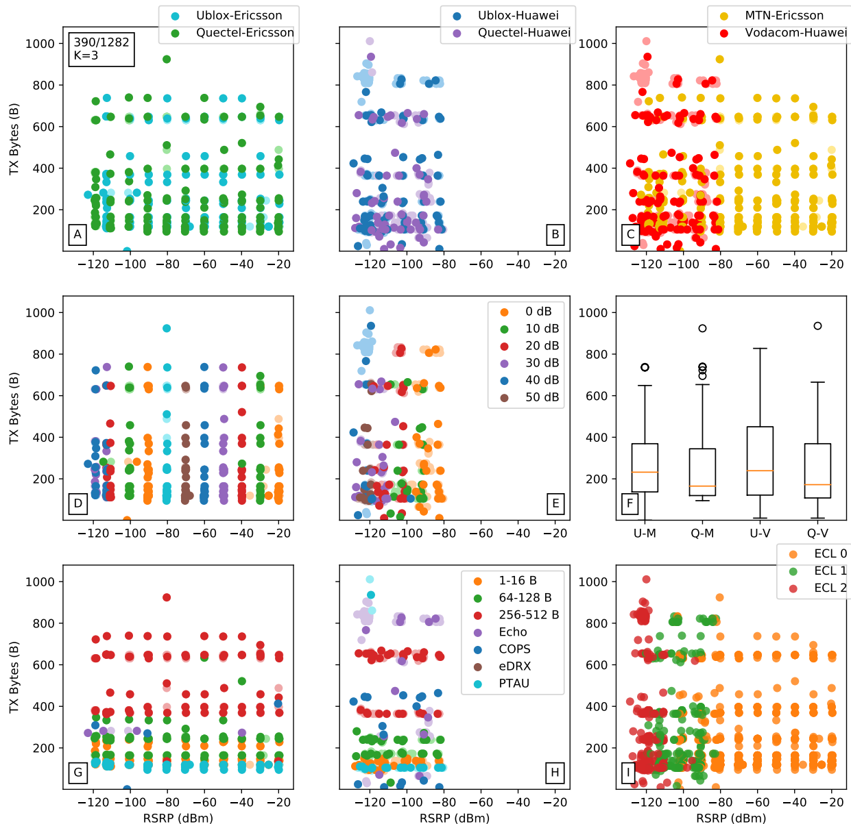
Figure C.20: TX packet sizes (390/1282) up to 1kB in comparison (AB) of UE, (C) MNOS, (DE) attenuation zones, (F) UE-MNO boxplots, (GH) test types, (I) and ECLs against RSRP. Attenuation zones evident and do not affect packet size. UE-MNO pairs share similar characteristics. Different tests are grouped with similar sizes with UDP packets being the largest, and COPS the smallest. ECL does seem to affect packet size.
