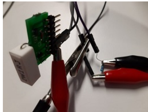
(b) ZXCT1008 high-side current monitor in action
