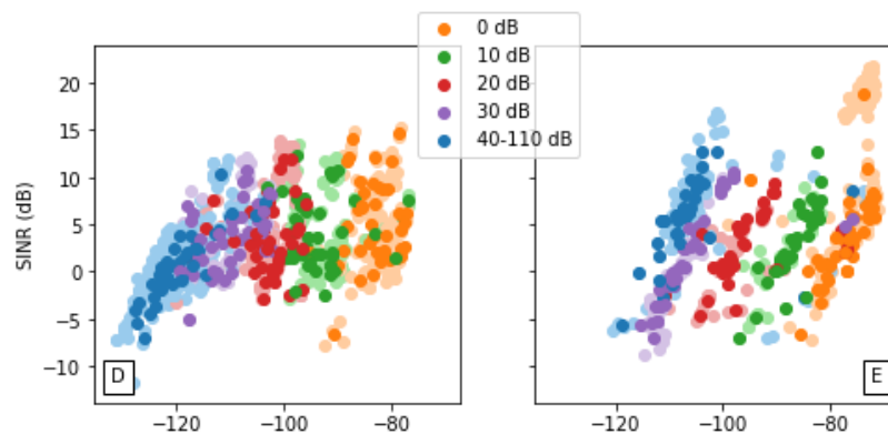
Figure 3.34: SINR against RSRP for Ublox and Quectel devices (relatively similar for now, thus combined) on MTN-ZTE (left) and Vodacom-Nokia (right). Each attenuation zone shows similar ranges of SINR, thus not as useful as RSRP when comparing other metrics against it. Ideally it should show a more linear relationship, and it is possible that these SINR readings are not accurate and contributing to variations in measured metrics.
