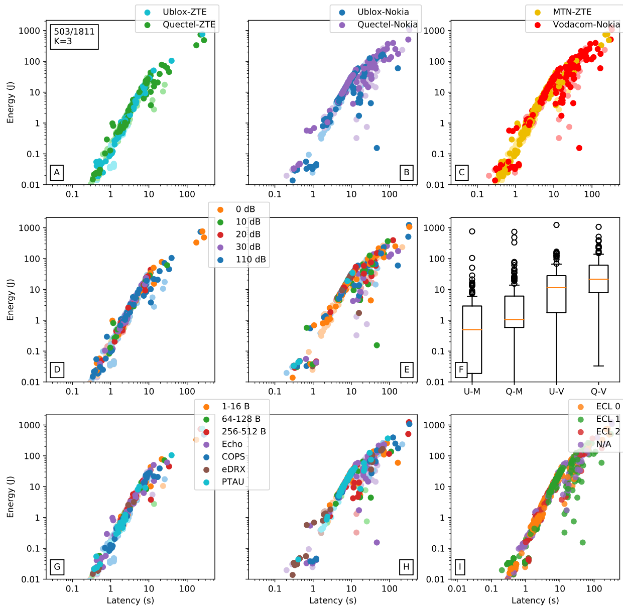
Figure C.9: Energy versus latency packets (503/1811) in comparison (AB) of UE, (C) MNOs, (DE) attenuation zones, (F) UE-MNO boxplots, (GH) test types, (I) and ECLs against RSRP for ZTE, Nokia.
