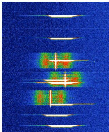
Figure 3.11: SigFox and LoRa RF signals @868 MHz on a waterfall diagram, with the x-axis showing frequencies at 868 MHz and the y-axis over time. The SigFox signals (vertical) take about 2 seconds to transmit, and the LoRa signals (horizontal) take a few hundred milliseconds.
