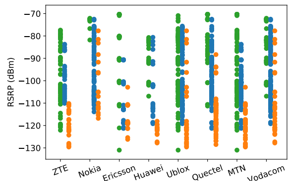
(b) The figure shows the distribution of ECL classes against RSRP. Transitions between ECL classes vary between LTE vendors depending on their network configuration and possibly another factor, as there is significant overlap between ECL class 0 and 1. ECL class 2 is more well defined, existing from roughly -110 dBm to -130 dBm, except for Nokia which shows values up to -80 dBm.
