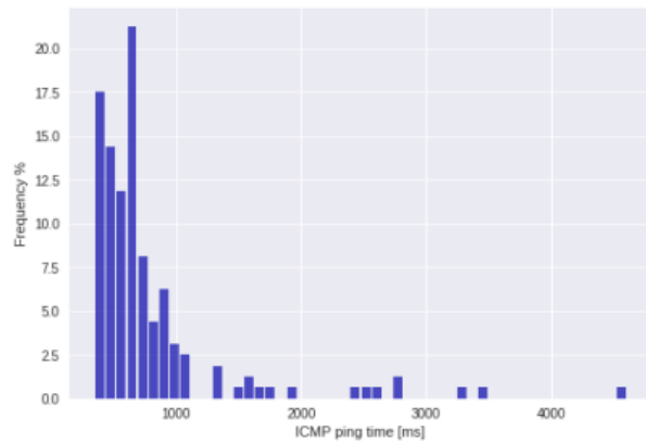
(a) 20 dB attenuation test in Technopark at -107 dBm RSRP in ECL 2. At 20dB attenuation, the data is more spread across 350 - 1000ms with a mean of 793.4ms and a tail that extends to over 4500ms. Any more attenuation and the signal is lost.
