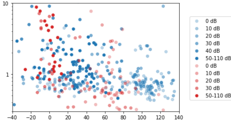
Figure 3.25: Ublox (blue) and Quectel (red) energy (mJ) per datagram as a function of the SINR (dB) as reported by the UE on the MTN-ZTE network. Increasing the range fully and using logarithms in Fig. 3.25, one can see that there is significant overshoot on the MTN-ZTE network. The trend mentioned in Fig. 3.24 continues.
