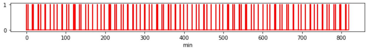
Figure 3.13: This test shows eDRX events until 800 minutes, measured externally. It shows an irregular eDRX time when not properly configured.
