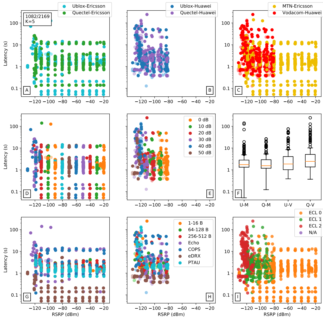
Figure C.2: Latency points (1082/2169) in comparison (AB) of UE, (C) MNOs, (DE) attenuation zones, (F) UE-MNO boxplots, (GH) test types, (I) and ECLs against RSRP for Huawei, Ericsson. In Figure C.2, variability between Quectel Ublox differs slightly, else they share similar traits. Ericsson shows slightly less latency on the MTN network.
