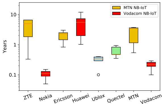
(a) The figure shows battery longevity estimations using energy measurements from Appendix A up to 10 years. ZTE, Ericsson and Huawei show results distributed roughly between 1 to 10 years, while Nokia sits between 2 to 8 weeks. In these measured estimations, the Quectel modem shows better values than the Ublox modem.
