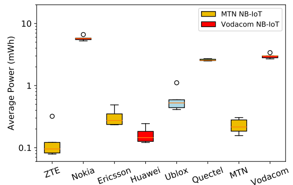
(b) The figure shows estimated average power distribution in ECL class 1 with mean dataset as shown in Appendix B
