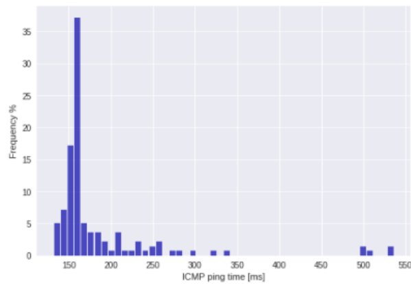
(a) 0 dB attenuation test in ECL class 0 at -51 dBm RSRP. With an antenna and the attenuator set to 0dB, we find most of the values around the mean of 185.2ms, except for the tail at around 500ms which is the time of the first ping in a set of 10.
