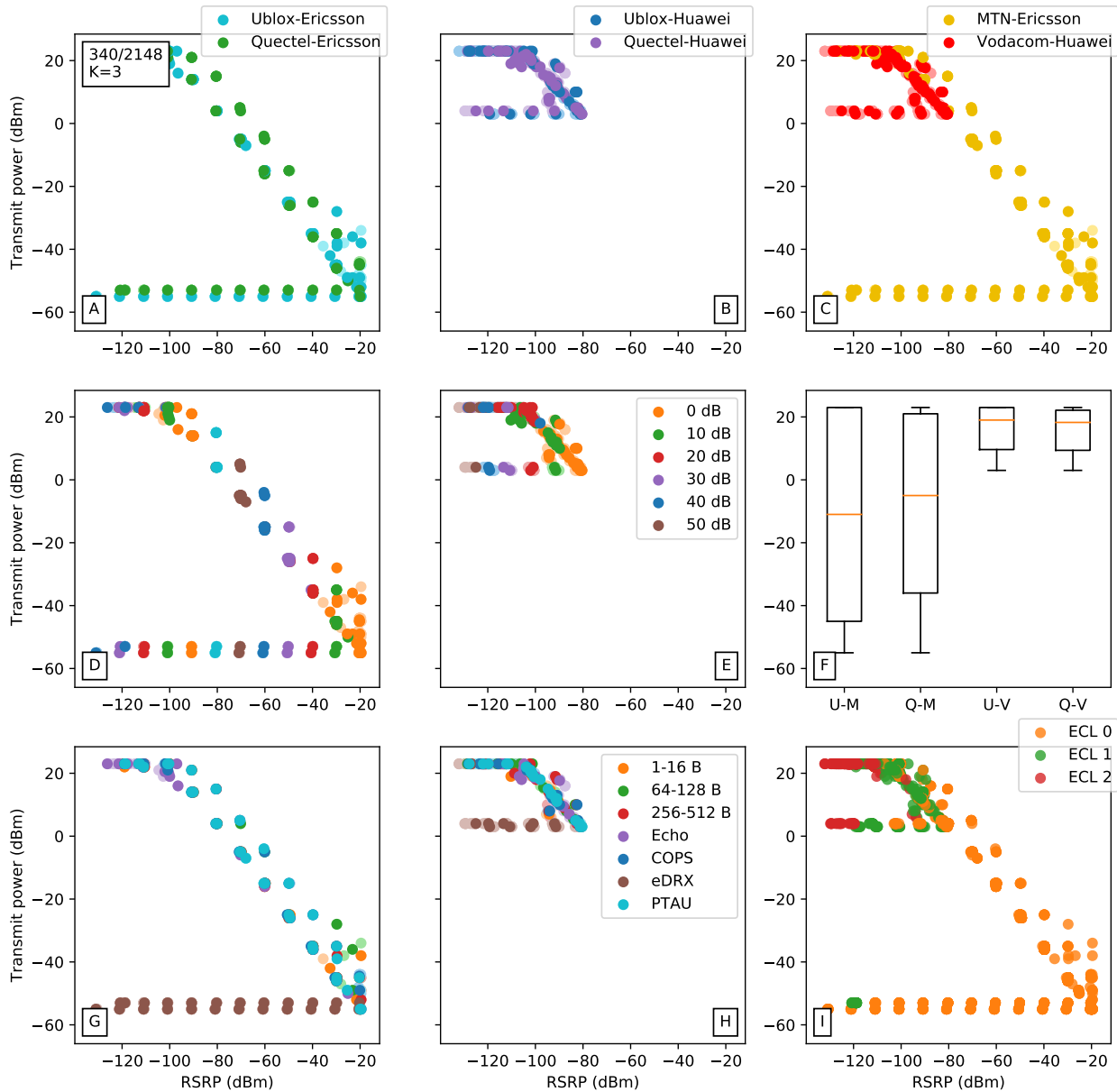
Figure C.14: Transmit powers of packets (340/2148) from -60 to 23 dBm in comparison (AB) of UE, (C) MNOs, (DE) attenuation zones, (F) UE-MNO boxplots, (GH) test types, (I) and ECLs against RSRP Ericsson, Huawei.
