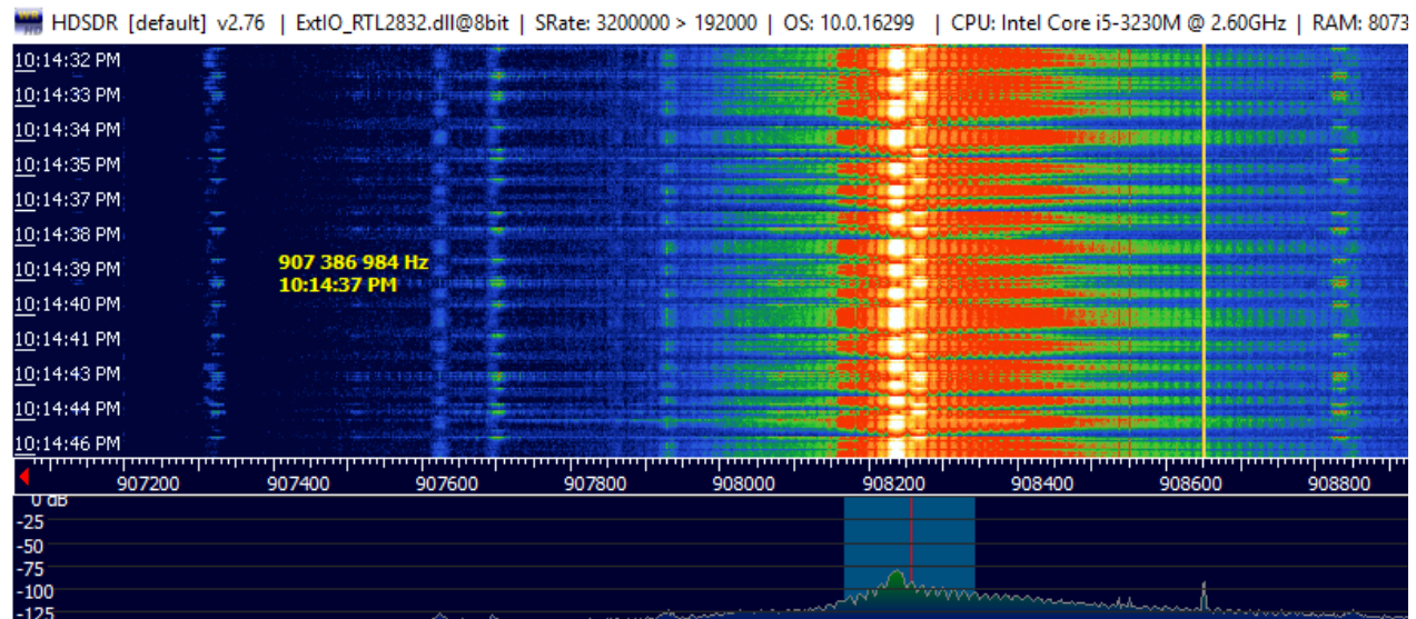
Figure F.1: Retry transmit signals for the WP7702 when extremely close to the edge of signal strength and outside the 180kHz bandwidth channel.
