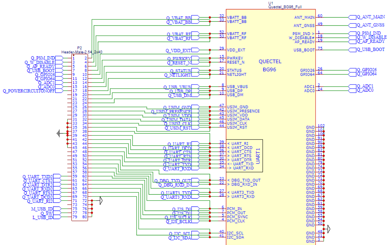
Figure D.1: Quectel BG96 modem schematic
