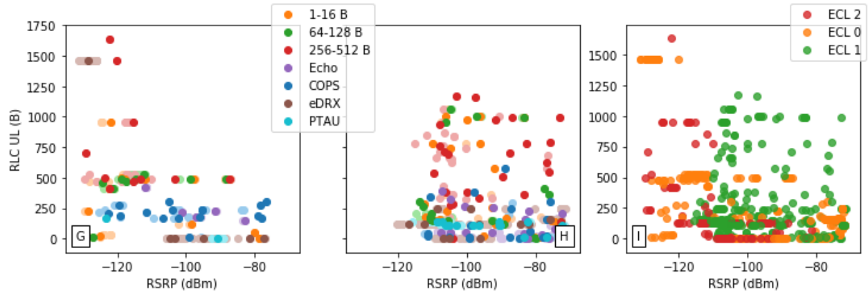
Figure C.16: Snippet of RLC UL throughput
