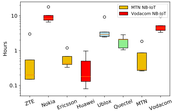
(a) The figure shows estimated telemetry interval using energy measurements from Appendix A. ZTE, Ericsson and Huawei require messages to be sent within every 5 minutes to an hour to last a year on a 9.36 Wh battery (AA-sized), while Nokia requires a telemetry interval around 10 hours. In these measured estimations, Quectel shows better values than Ublox.
