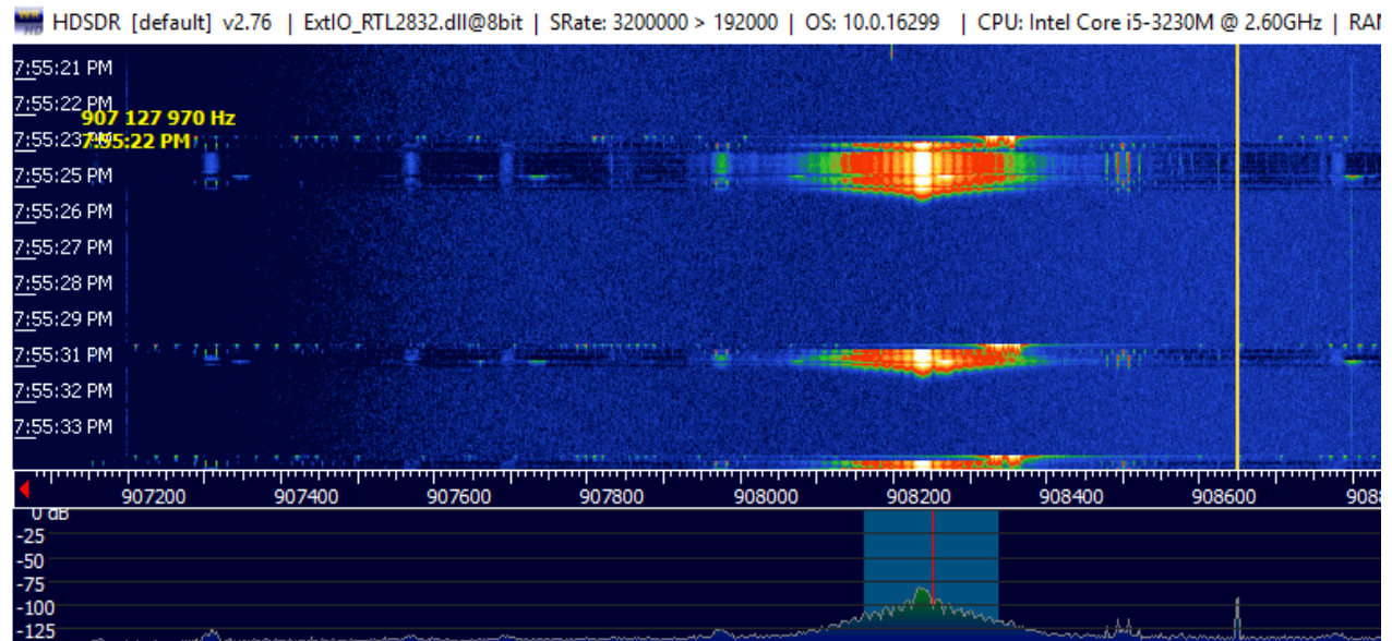
Figure 3.10: 5 dB SINR NB-IoT transmissions using Sierra Wireless WP7702 at 908.2 MHz and EARFCN 3734 of length 2282ms, 1560ms and 1380ms respectively.
