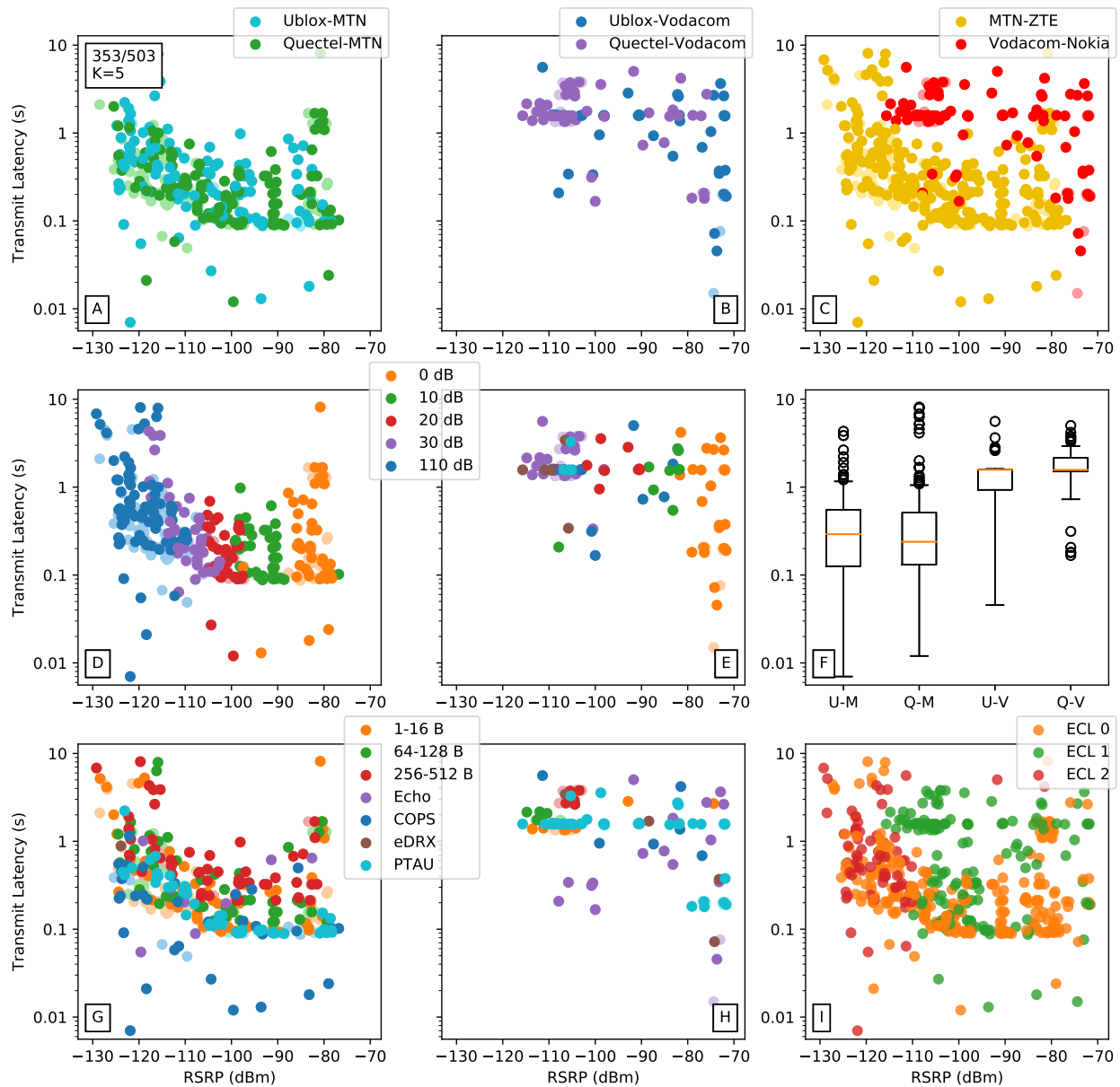
Figure C.3: TX time points (353/503) in comparison (AB) of UE, (C) MNOs, (DE) attenuation zones, (F) UE-MNO boxplots, (GH) test types, (I) and ECLs against RSRP for ZTE, Nokia.
