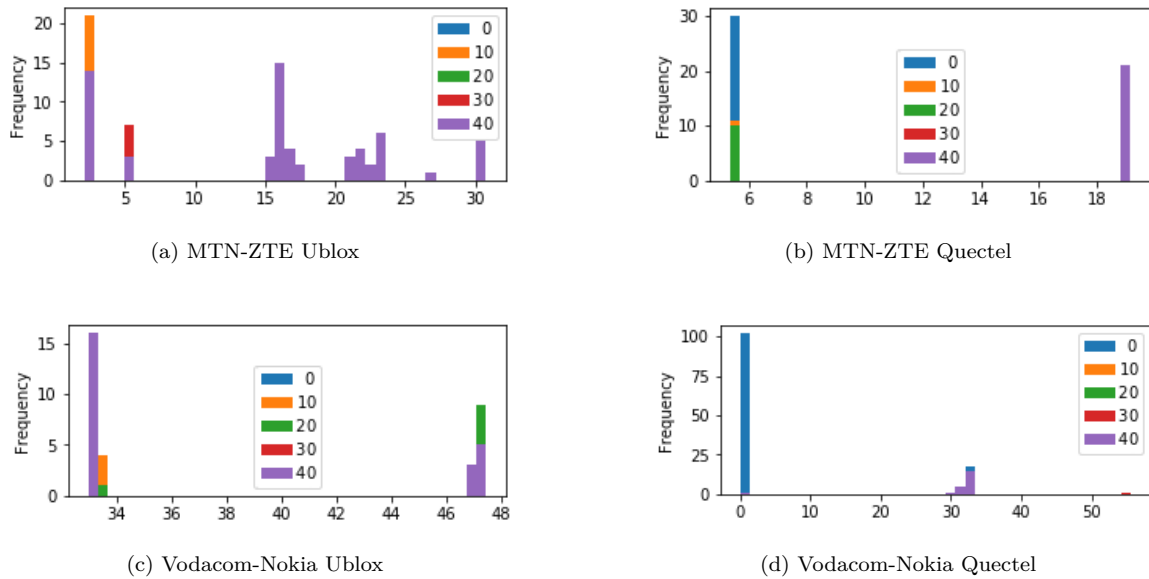
Figure 3.28: eDRX histograms of the energy produced by listening for paging occasions with respect to RF attenuation in dBm as mentioned in §2.5.5.3. Martinez [3] measured values under 10mJ for both Ublox and Quectel, yet on the MTN-ZTE and Vodacom-Nokia networks it is up to 5 times more. Thus, it is apparent that network configuration is the cause of these differences.
