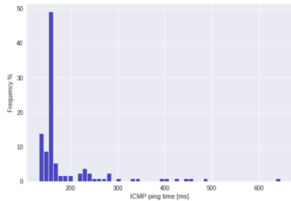
(b) 110 dB attenuation test in ECL 0, at -85 dBm RSRP. Setting the attenuator to the max of 110dB, we see no change in the ping measurements which have a mean of 185.9ms. The tail has increased to a max of just over 600ms.
