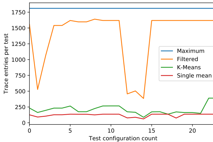
Figure 3.40: Trace entries per test (CSV file). In this example, the absolute maximum of 1811 traces has been filtered by removing duplicates and applying thresholds. K-means clustering achieves the desired effect of reducing dimensionality and skewness induced from low latency sampling on the dataset for different tests, yet keeps most of the features of the thresholded max. This allows for easier visualization and unbiased feature comparison.
