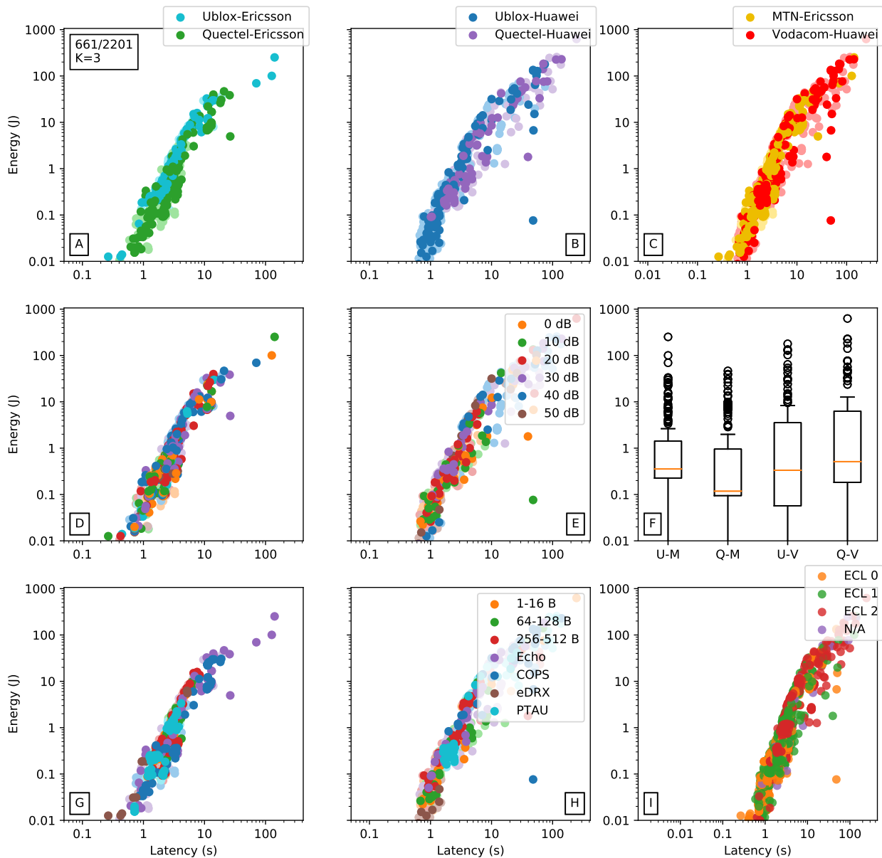
Figure C.10: Energy versus latency packets (661/2201) in comparison (AB) of UE, (C) MNOs, (DE) attenuation zones, (F) UE-MNO boxplots, (GH) test types, (I) and ECLs against RSRP for Ericsson, Huawei.
