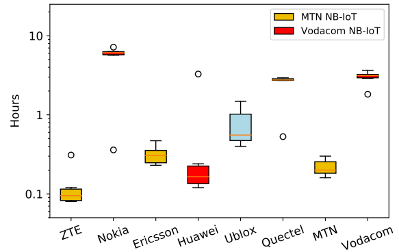
(b) The figure shows telemetry interval estimations for UE reported RF time from Appendix B. ZTE, Ericsson and Huawei require messages to be sent within every 5 to 30 minutes, while Nokia expects a telemetry interval every 6 hours. In these estimations from UE reports, the Ublox modem is shown to be better than the Quectel modem.
