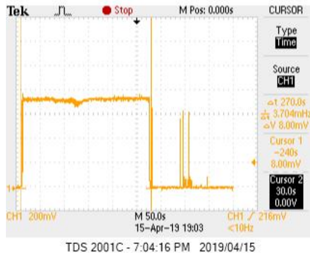
Figure 3.22: AT+COPS=0 network registration on MTN-ZTE network with lengthy inactivity timer setting of 270s.
