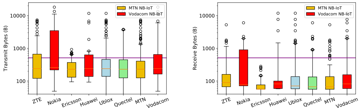
(a) Transmission bytes of all manufacturers and operators, with at least 50% of values centered between 100 and 1000 bytes except for Nokia which extends further, having a 95th percentile at 10,000 bytes or more in outliers.
