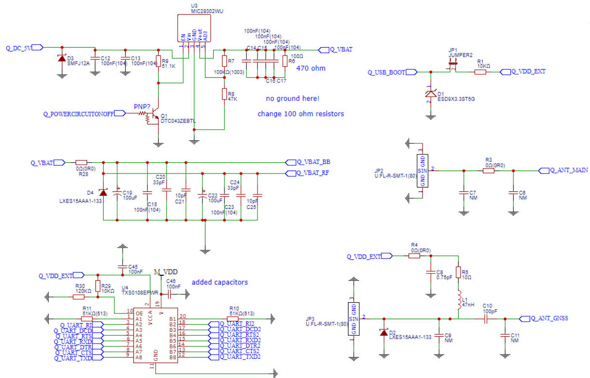
Figure D.3: Power circuitry, antenna and logic level conversion
