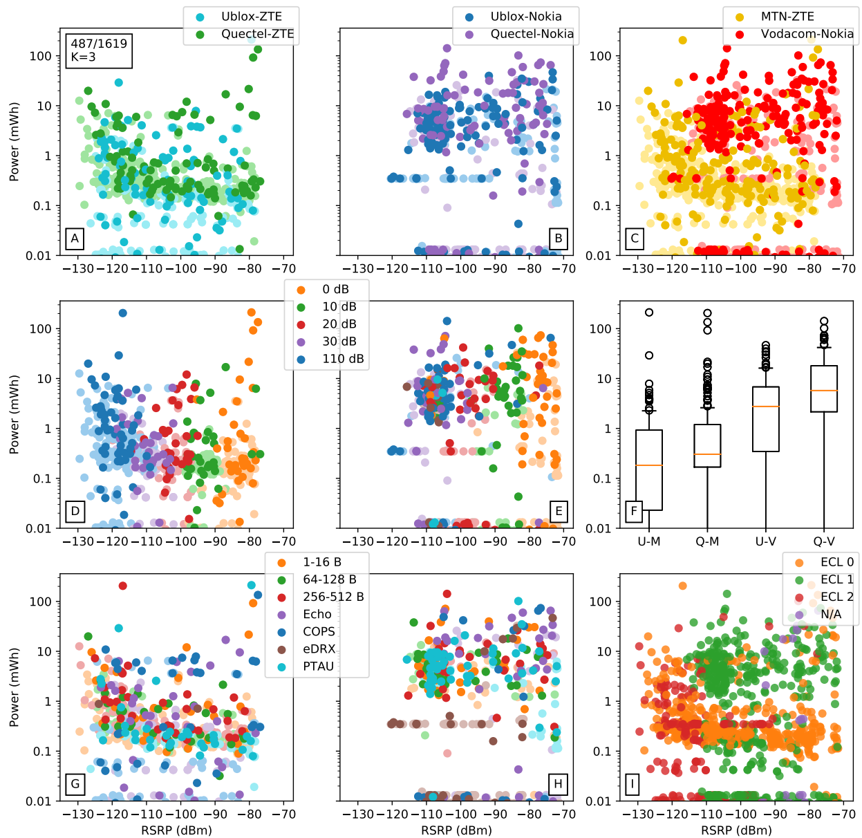
Figure C.7: Energy packets (487/1619) in comparison (AB) of UE, (C) MNOs, (DE) attenuation zones, (F) UE-MNO boxplots, (GH) test types, (I) and ECLs against RSRP for ZTE, Nokia.
