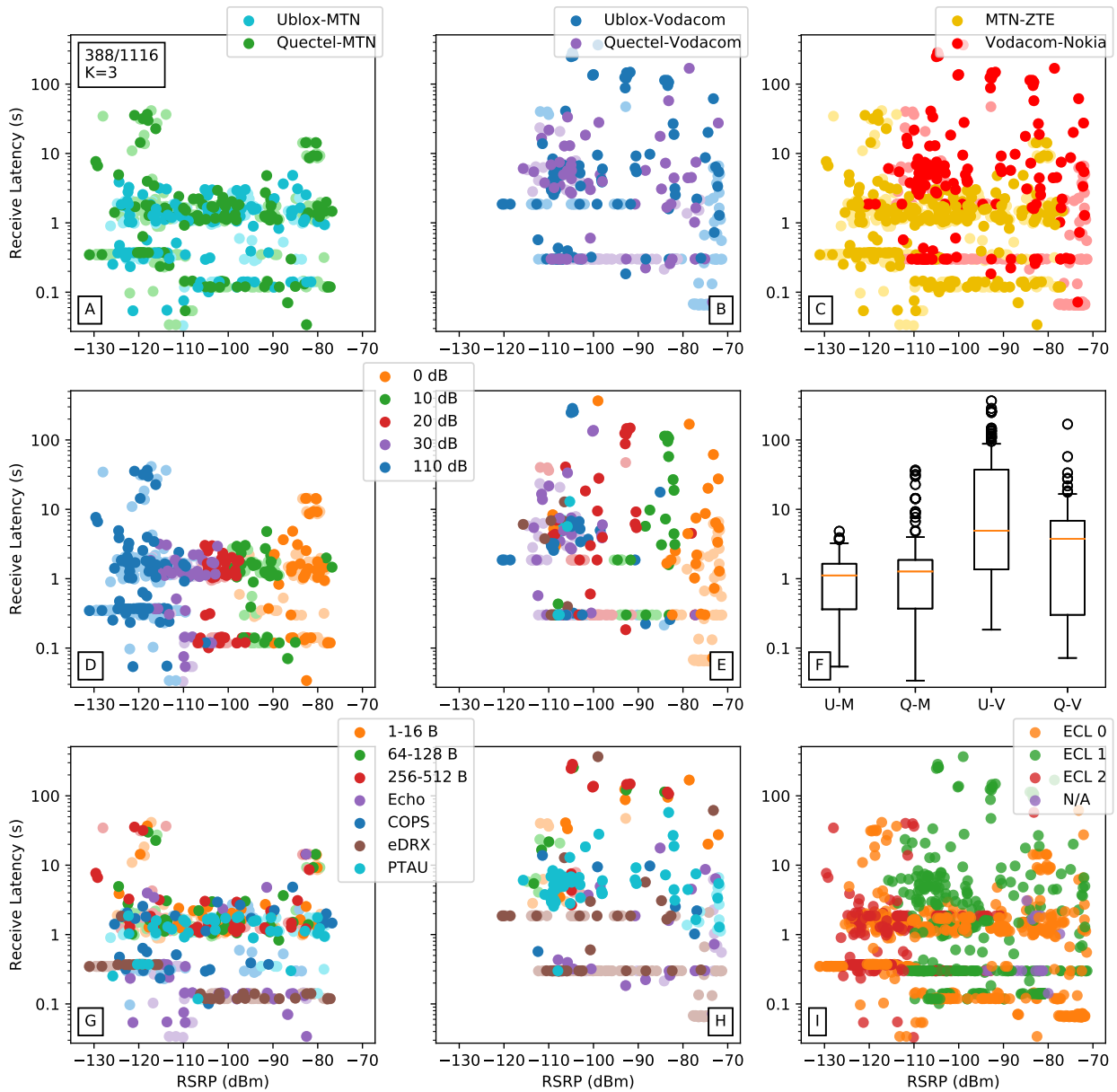
Figure C.5: RX time packets (388/1116) in comparison (AB) of UE, (C) MNOs, (DE) attenuation zones, (F) UE-MNO boxplots, (GH) test types, (I) and ECLs against RSRP for ZTE, Nokia.
