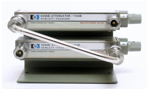
Figure 3.17: The Hewlett Packard attenuators used in this study to change the RF conditions for UE devices against multiple LTE vendors
