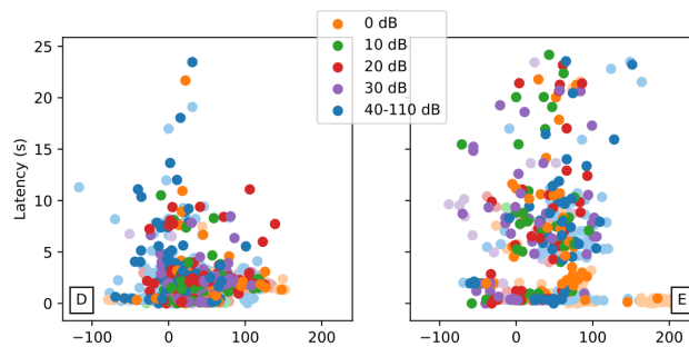
Figure 3.30: Latency per datagram as a function of the SINR (dB) as reported by the UE on the (D) MTN-ZTE and (E) Vodacom-Nokia network respectively. In Fig. 3.30, there is a poor distinction between attenuation zones as the SINR varies throughout the reported RSRP range. Grouping the data according to attenuation decade is important to see the effect of network conditions clearly.
