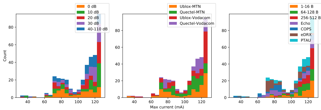
Figure 3.27: Peak energy measurements from roughly 70mA and skewed towards 128mA. These high peak energies shouldn't affect the average power much as peak current occurs only during the first few microseconds of the random access preamble (PRACH).
