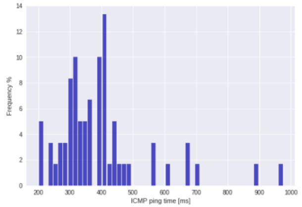
(b) 10 dB attenuation test in Technopark at -101 dBm RSRP in ECL class 1. In this condition, the data is more spread out from 200 - 500ms with a mean of 396.4ms and a tail at just under 1000ms.
