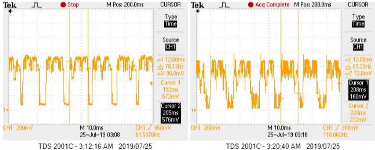
(a) C-DRX timing on MTN-ZTE-Ublox
