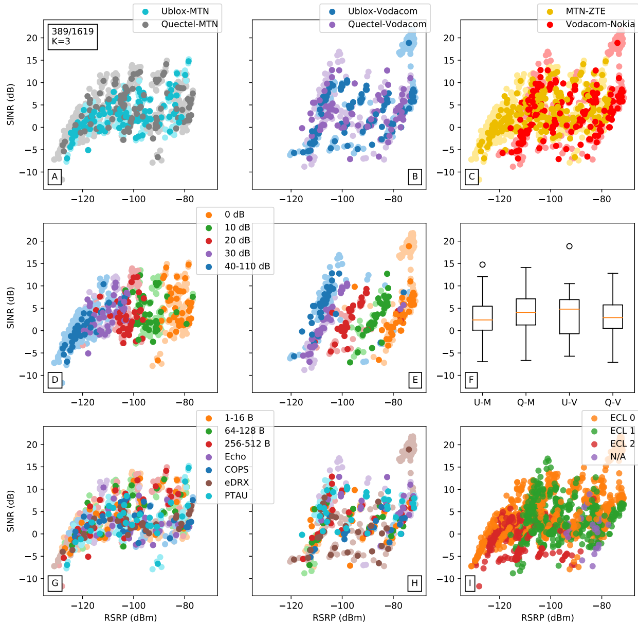
Figure C.12: SINR versus RSRP packets (389/1619) in comparison (AB) of UE, (C) MNOs, (DE) attenuation zones, (F) UE-MNO boxplots, (GH) test types, (I) and ECLs.
