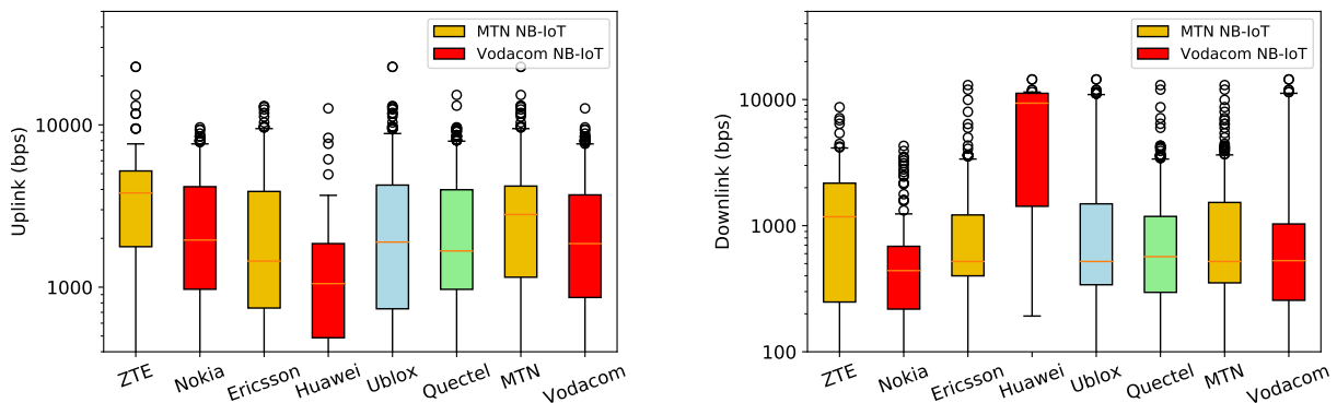
(a) The figure shows RLC and MAC uplink throughput, with 95% of values under 10 kbps. ZTE is performing best with a central tendency at 4 kbps, and Huawei the least at 1 kbps. It is shown that Nokia, Ericsson, Ublox, Quectel and Vodacom have similar central tendency distributions at 2 kbps, while MTN leads with 3 kbps.
