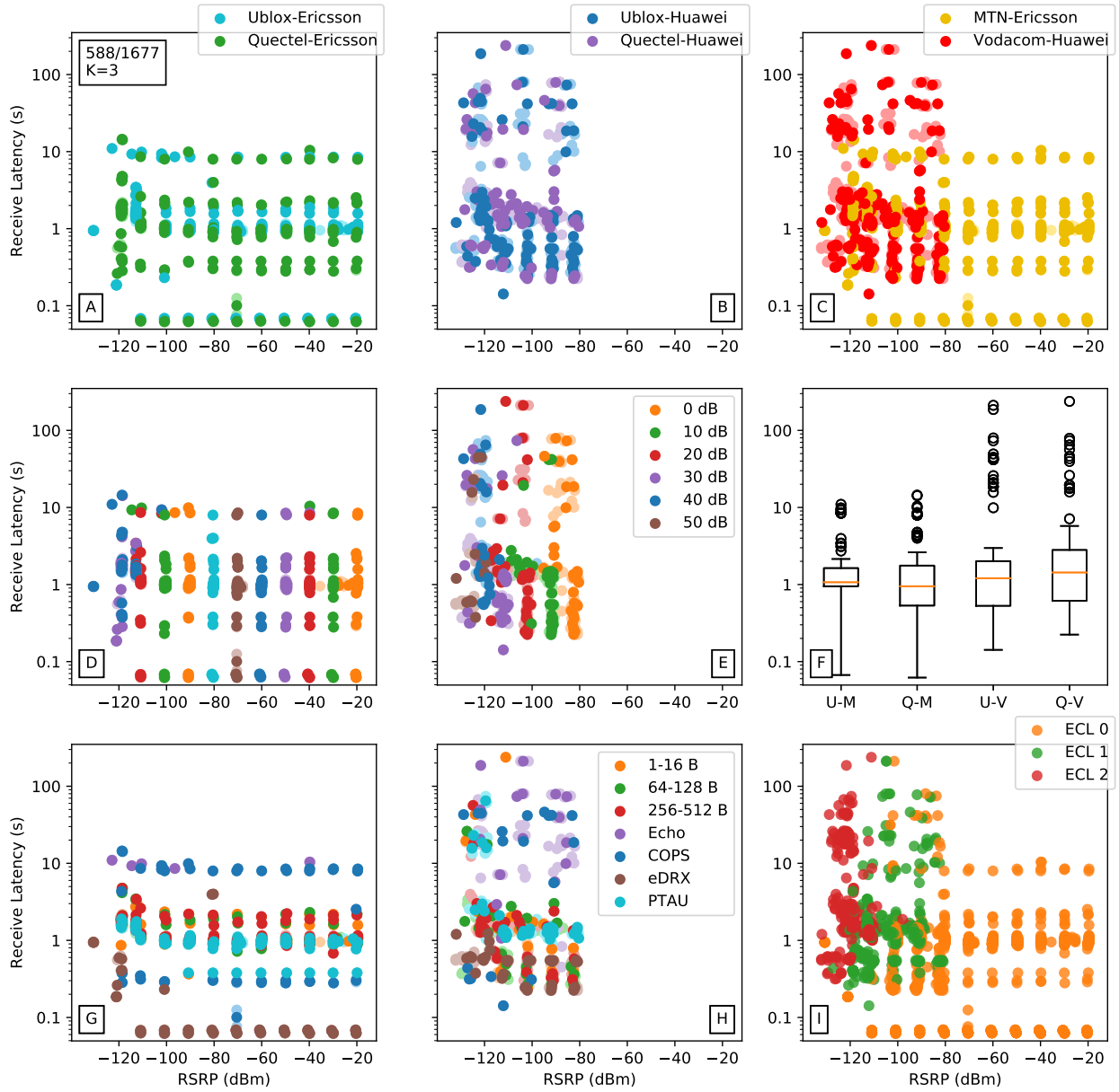
Figure C.6: RX time packets (588/1677) in comparison (AB) of UE, (C) MNOs, (DE) attenuation zones, (F) UE-MNO boxplots, (GH) test types, (I) and ECLs against RSRP for Ericsson, Huawei.
