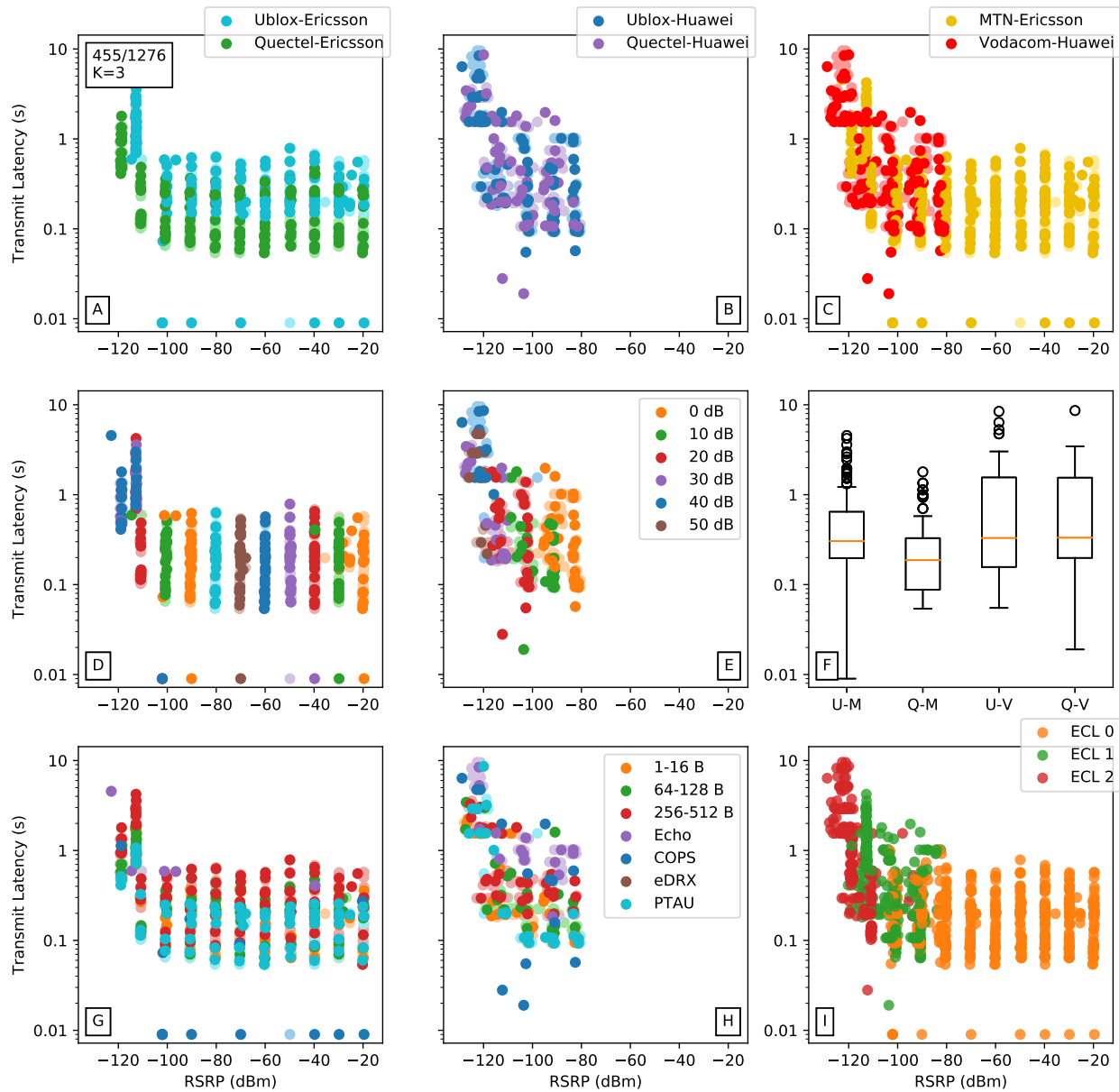
Figure C.4: TX time points (455/1276) in comparison (AB) of UE, (C) MNOs, (DE) attenuation zones, (F) UE-MNO boxplots, (GH) test types, (I) and ECLs against RSRP for Ericsson, Huawei.
