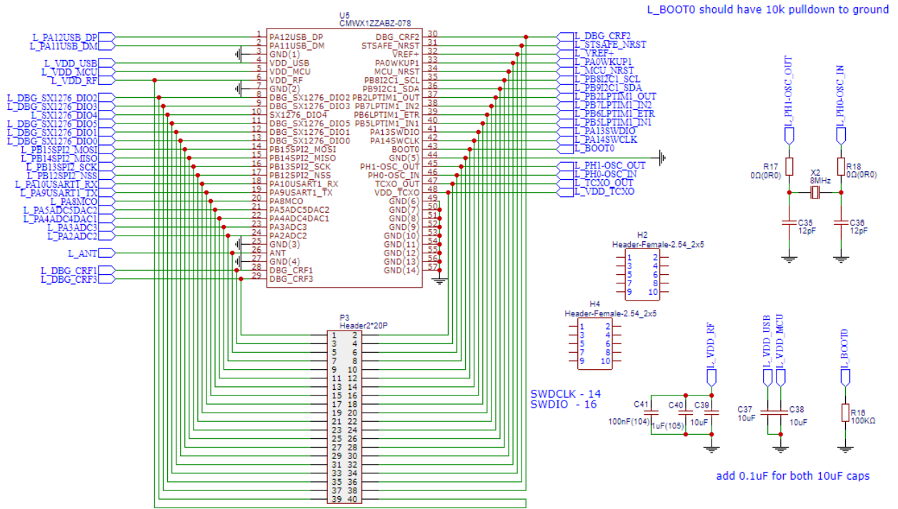
Figure D.4: Murata CMWX1ZZABZ-078 module schematic
