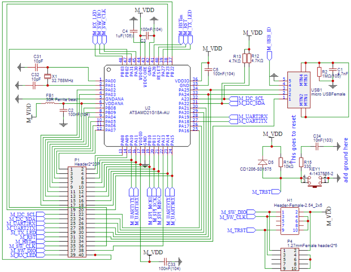
Figure D.5: Atmel ATSAMD21G18a microcontroller schematic
