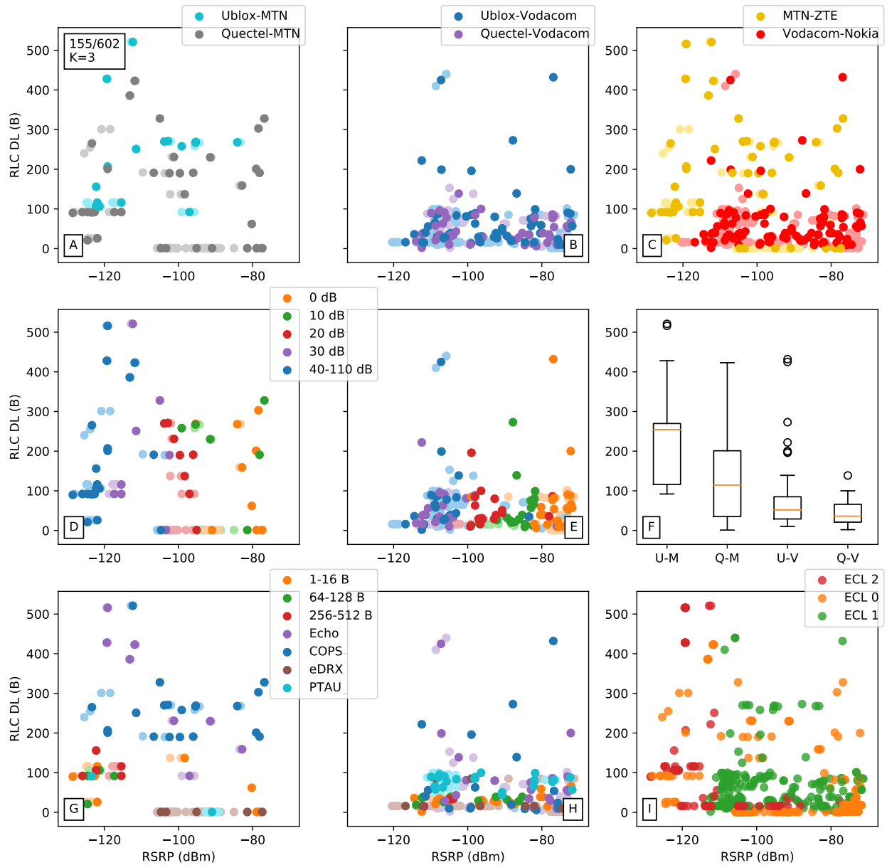
Figure C.15: RLC DL throughput of packets (155/602) in comparison (AB) of UE, (C) MNOs, (DE) attenuation zones, (F) UE-MNO boxplots, (GH) test types, (I) and ECLs against RSRP for ZTE, Nokia.
