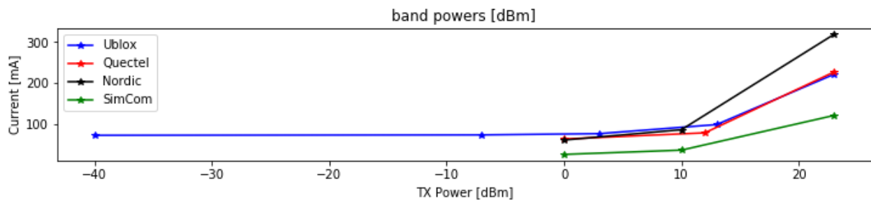
Figure 2.10: This diagram shows how current versus transmit power for NB-IoT modems remains stable under 0 dBm and increases exponentially until 23 dBm.
