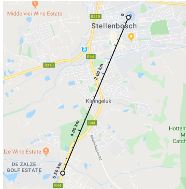
(b) The greatest distance measured was 5.5km from the intersection of the R44 and the turn-off to Stellenbosch Square or Jamestown at an altitude of 106m. This is a relative elevation of -32m to the base station and at an RSRP of -89dBm.
