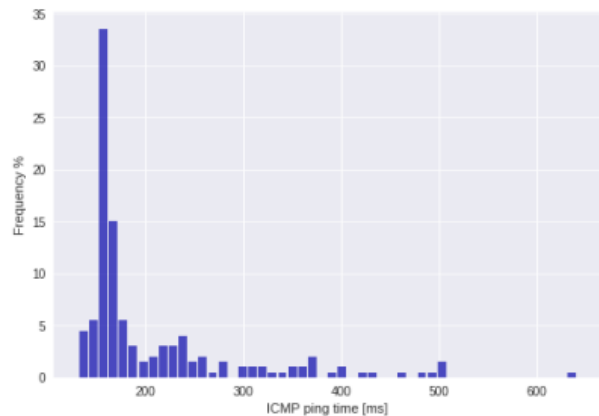
(c) Attenuator and no antenna test in ECL 0 at -91 dBm RSRP. Removing the antenna from the attenuator, we find that the data has a slightly thicker tail, and averages around 207.1ms.
