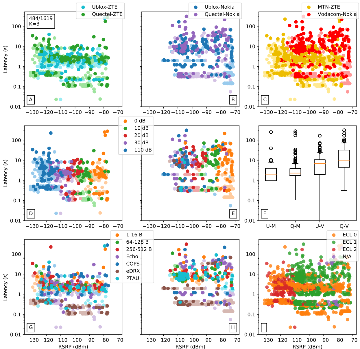
Figure C.1: Latency points (484/1619) in comparison (AB) of UE, (C) MNOs, (DE) attenuation zones, (F) UE-MNO boxplots, (GH) test types, (I) and ECLs against RSRP for ZTE, Nokia.
