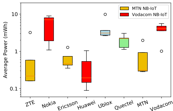
(a) The figure shows measured average power distribution in ECL class 1 with mean dataset as shown in Appendix A
