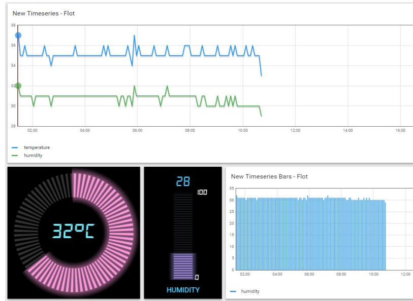
Figure 3.16: Dashboard showing communication between NB-IoT PCB and Thingsboard cloud via MQTT with temperature, humidity, push button and downlink buzzer control
