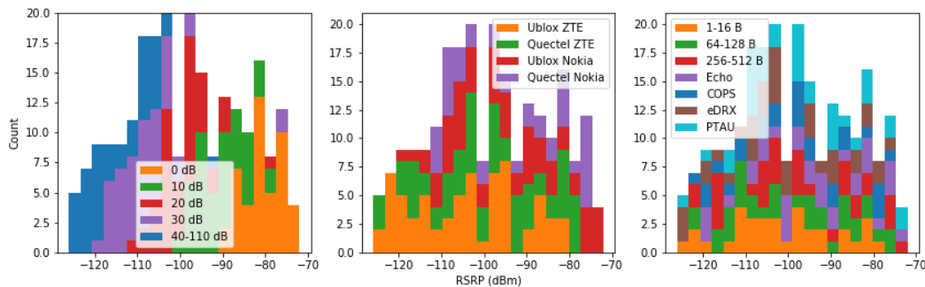
Figure 3.32: RSRP distribution using Ublox and Quectel UE on ZTE-MTN and Nokia-Vodacom infrastructure as well as attenuation and telemetry test set. RSRP and telemetry tests have a relatively even distribution, although RSRP still has about 20 dBm variability per attenuation decade. ZTE signals have higher MCL than Nokia.
