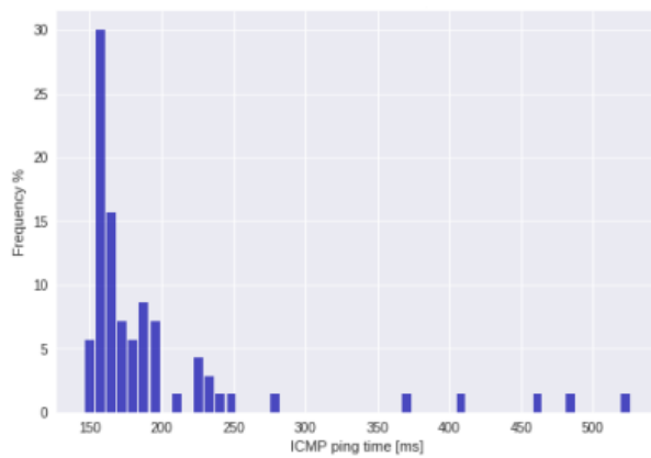
(a) 0 dB attenuation test in Technopark at -93 dBm RSRP in ECL class 0. With no attenuation, the data has a mean of 196.7ms and a tail just above 500ms.
