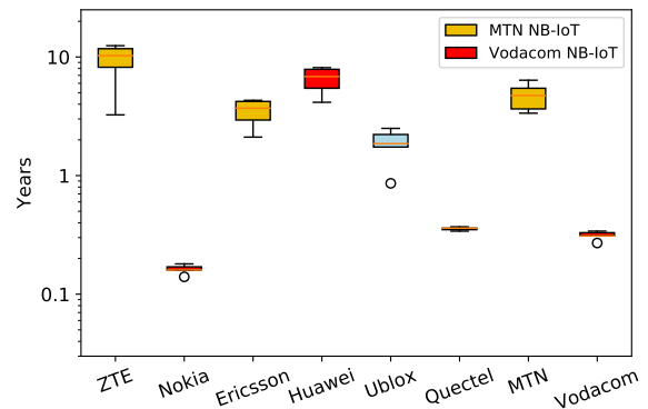
(b) The figure shows UE reported RF time from Appendix B up to 10 years. ZTE, Ericsson and Huawei show results distributed roughly between 2 to 10 years, while Nokia sits at around 8 weeks. In these estimations from UE reports, the Ublox modem is shown to be better than the Quectel modem.
