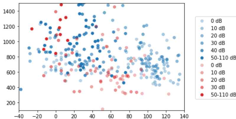
Figure 3.24: Ublox (blue) and Quectel (red) energy (J) per datagram as a function of the SINR (dB) as reported by the UE on the MTN-ZTE network limited to 1500 mJ. With the fading colour scheme and range just as in Martinez [2], Fig. 3.24 shows the impact of SNR on energy consumption. As observed in the figure, there is a trend of increasing energy with respect to lower SNR levels and high variability. Unfortunately, the effect of different ECLs is unclear.
