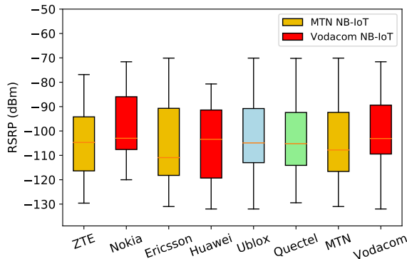
(a) The figure shows UE reported RSRP. Although Ericsson’s RSRP extended up to -20 dBm due to laboratory conditions, it is limited to -70 dBm. LTE vendors have similar values at -130 dBm, except for Nokia at -120 dBm, with approximate minimum values shown in Table 24.
