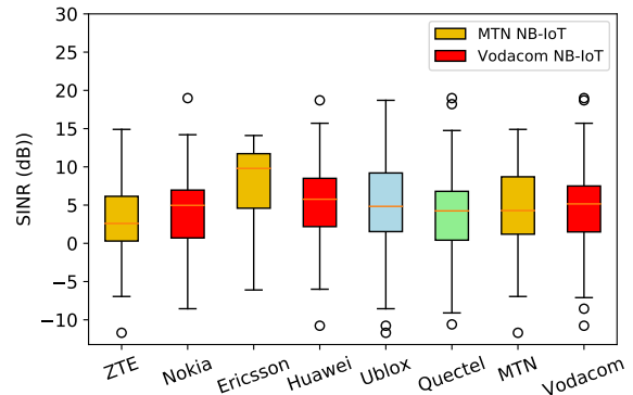
(b) With respect to LTE vendors, SINR is reported to be approximately from -7 dB to 15 dB, with approximate minimum values shown in Table 23. SINR values are more evenly distributed than RSRP, yet with more outliers.
