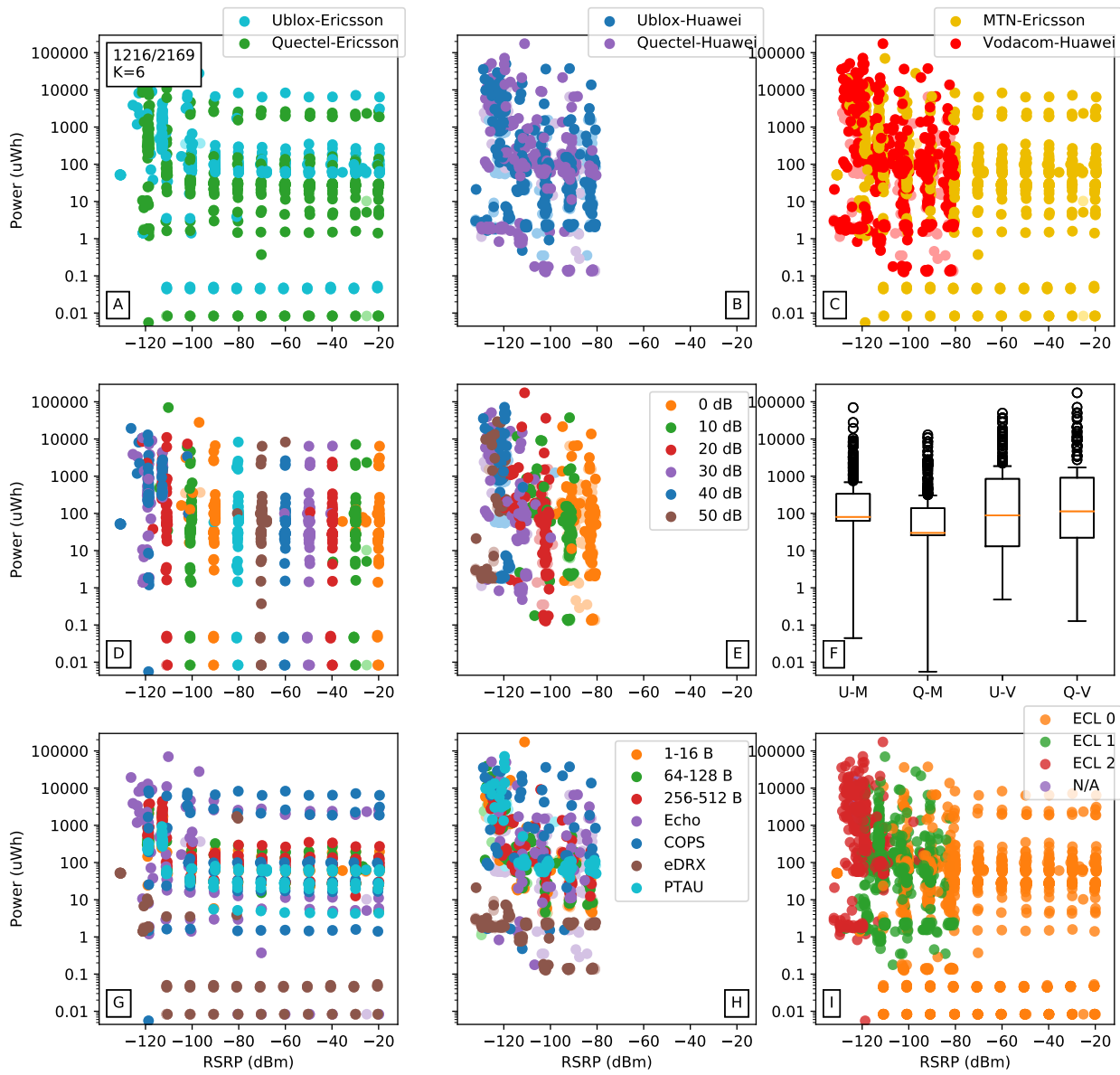
Figure C.8: Energy packets (1216/2169) in comparison (AB) of UE, (C) MNOs, (DE) attenuation zones, (F) UE-MNO boxplots, (GH) test types, (I) and ECLs against RSRP for Ericsson, Huawei.
