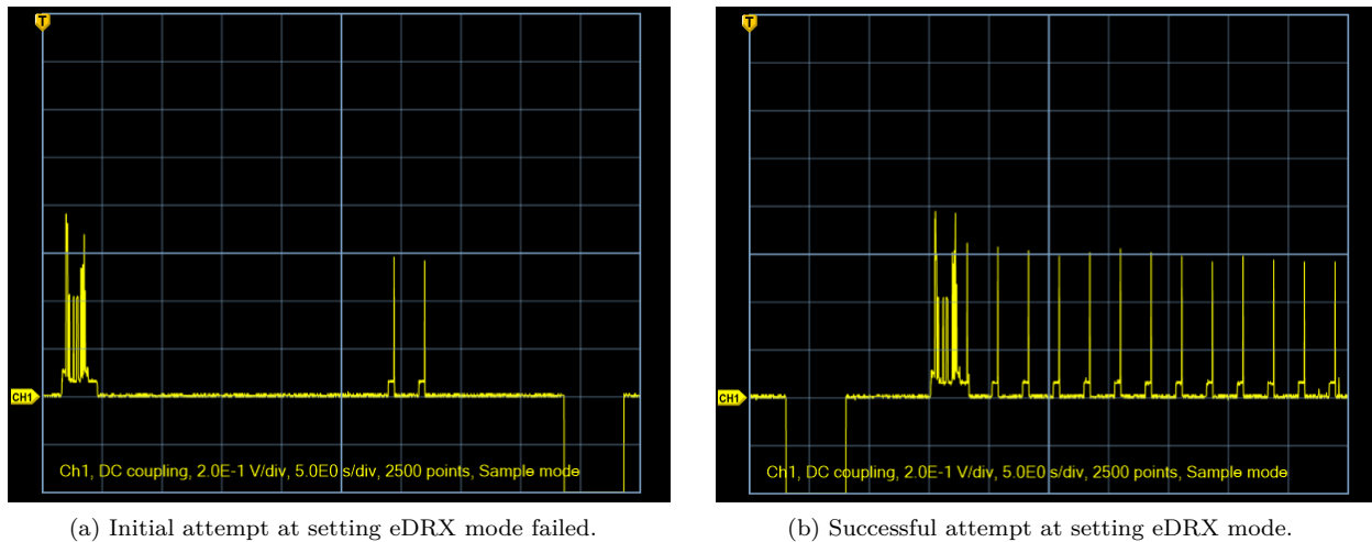
Figure 3.12: eDRX tests
