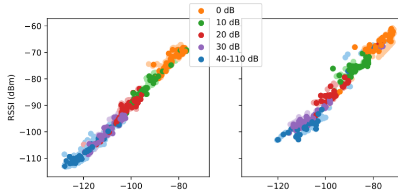
Figure 3.33: RSSI against RSRP for Ublox and Quectel devices (similar, thus combined) on MTN-ZTE (left) and Vodacom-Nokia (right). RSSI has a shorter ‘range’ than RSRP due to transmit power being included, and thus more information can be observed when comparing metrics against RSRP.
