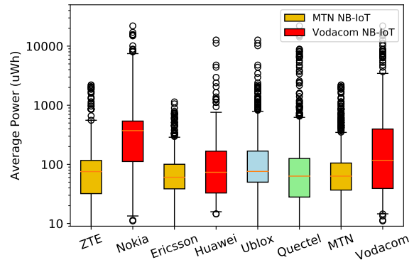
(b) The figure shows UE reported average power estimation distribution using transmit and receive time dataset as shown in Appendix C.1.2 and C.1.3.
