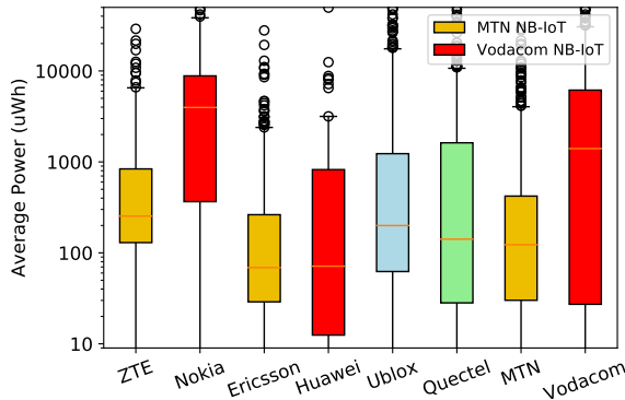
(a) The figure shows measured average power distribution with dataset as shown in Appendix C.2.1.
