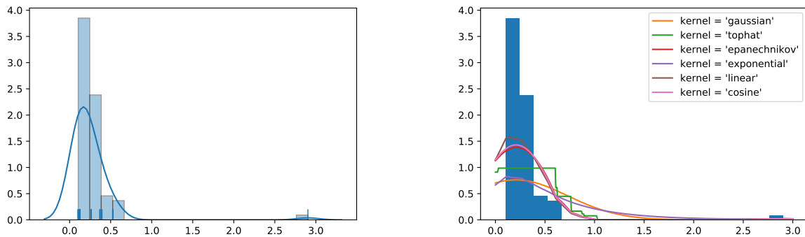
(a) The probability of the discrete data can be estimated in a continuous probability density function (PDF) with the kernel density estimation.
