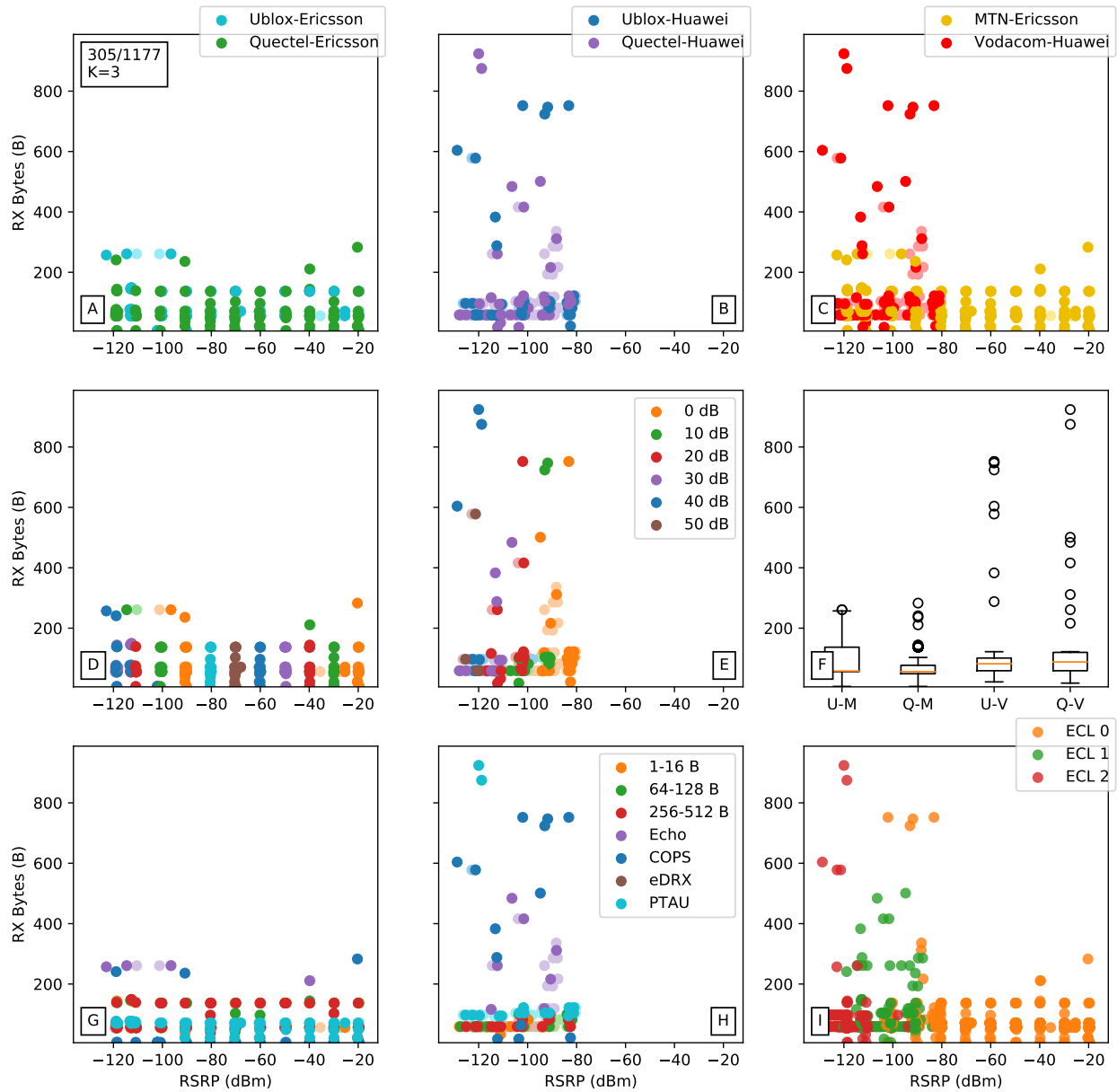
Figure C.22: RX packet sizes (305/1177) up to 200 bytes on average in comparison (AB) of UE, (C) MNOs, (DE) attenuation zones, (F) UE-MNO boxplots, (GH) test types, (I) and ECLs against RSRP. Attenuation zones evident and do not affect packet size. UE-MNO pairs share similar characteristics. Different tests are grouped with similar sizes with Echo, COPS and PTAU packets being the largest, and UDP the smallest. ECL does seem to affect packet size.
