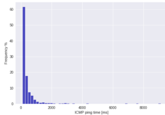
(b) Lastly, all the test data (including on the way to Technopark and back), we see a similar form except with a tail extending to almost 10 seconds, which is within 3GPP specifications.
