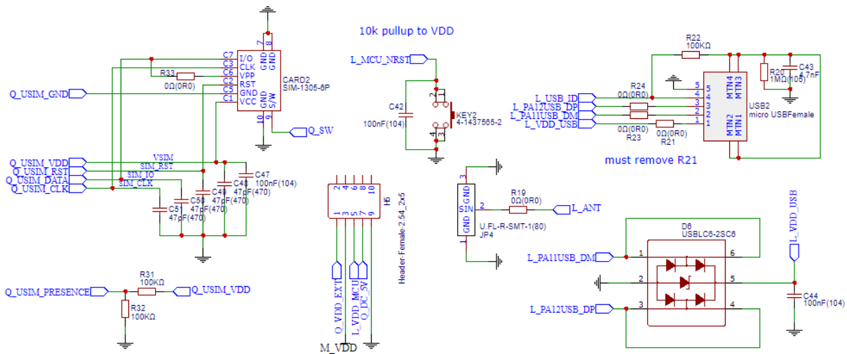
Figure D.2: SIM card, USB and miscellaneous circuitry schematic
