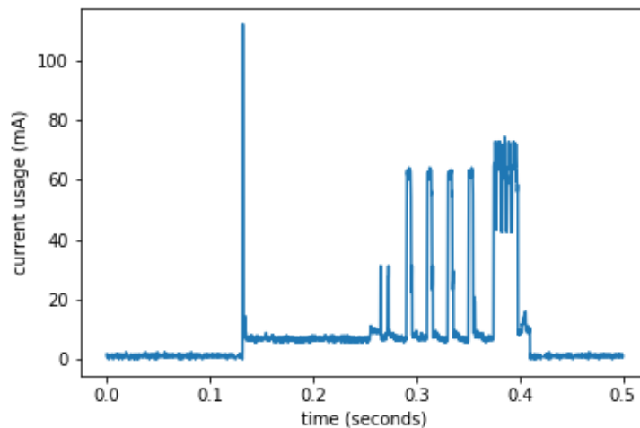
Figure 3.14: Typical eDRX current profile with a 277.8 ms duration. This shows how for the first few microseconds there is a large transmission current spike to synchronize, before receiving paging information from the cell tower.
