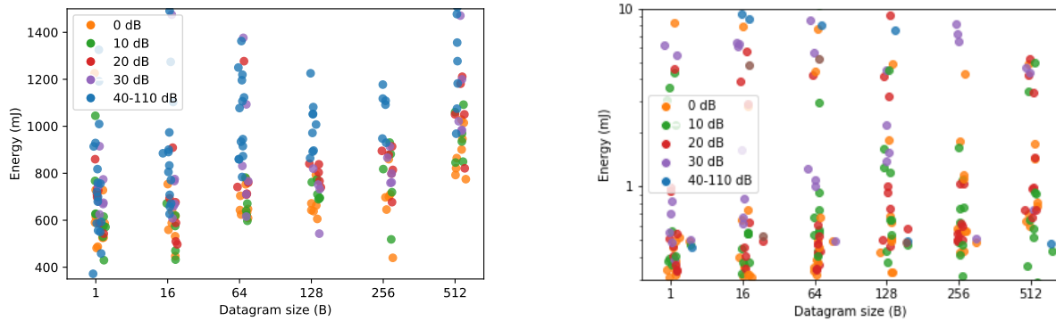
(a) Datagram sizes of MTN-Ublox pair up to 1500 mJ.
