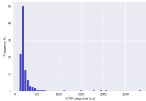
(a) 0 dB attenuation test at Parmalat at -87 dBm in ECL 0. A similar pattern was seen 3.0 km away from the base station at Parmalat, although driving closer there were a few spots where connection was lost or many retries were needed such that the tail extended up to almost 3000ms for the ICMP ping time.
