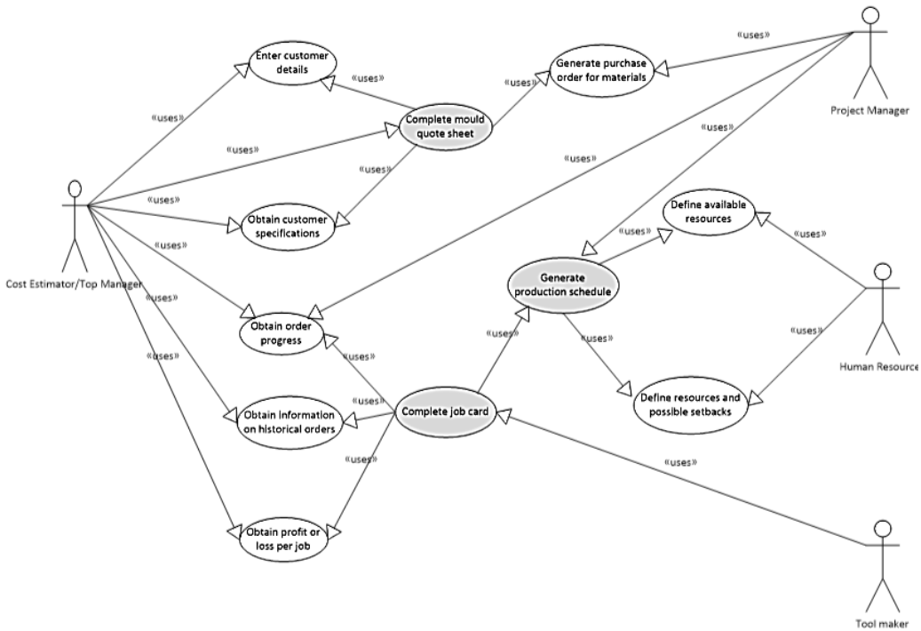
Figure 4: System use case model
