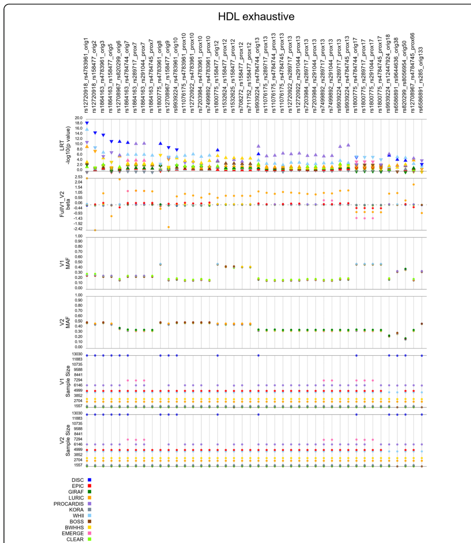
Fig. 4 Results for the main effect filter (MEF) analysis of HDL-C. Showing results for the models that passed the replication threshold of p < 3.0 \times 10^{-5} . Orig# and prox# designate models that were identified in the discovery cohort and those identified via proxy (i.e. both SNPs in high LD with SNPs from orig. Models), respectively. V1 and V2 are the two SNPs in the model; arrow in likelihood ratio test (LRT) row denotes direction of effect
