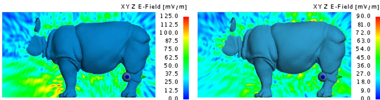
Figure 84: Electric field of the PIFA pair through the chest of the Shadwick [left] and weighted average [right] approximation models.
