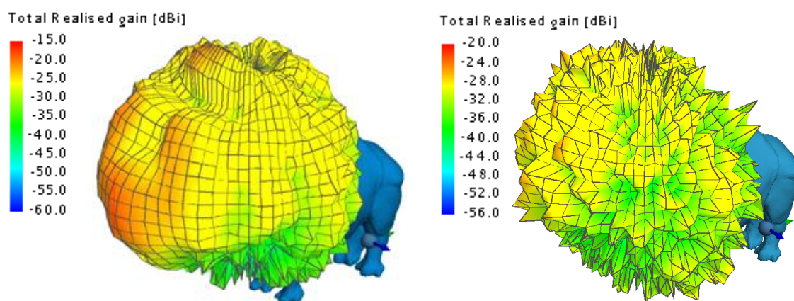
Figure 65: Realised gain of the Shadwick (left) and weighted average (right) anatomical rhinoceros back model [MFPEMA pair].
