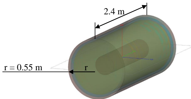
Figure 16: Layered cylindrical rhinoceros computer simulation model.
