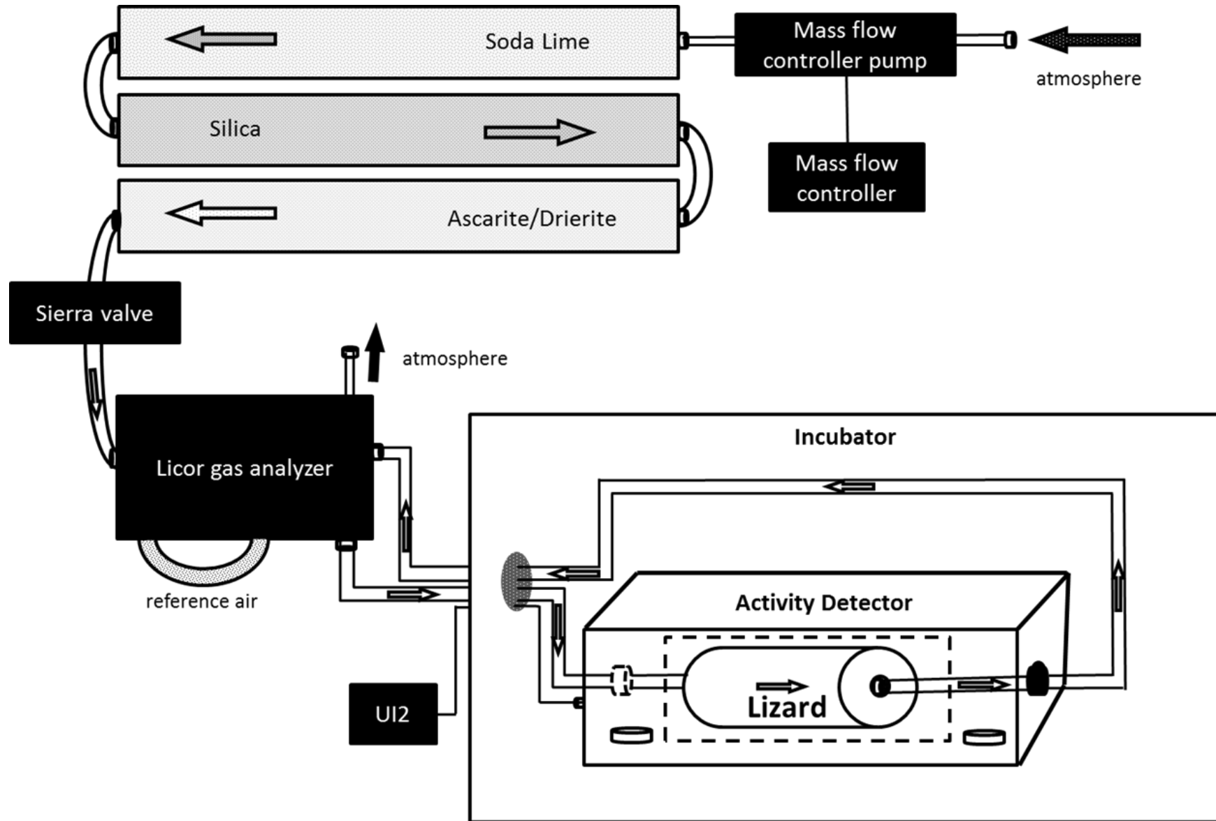
Appendix 1.4: Experimental set-up of flow through respirometry measurements to determine RMR and TEWL of Meroles knoxii .
